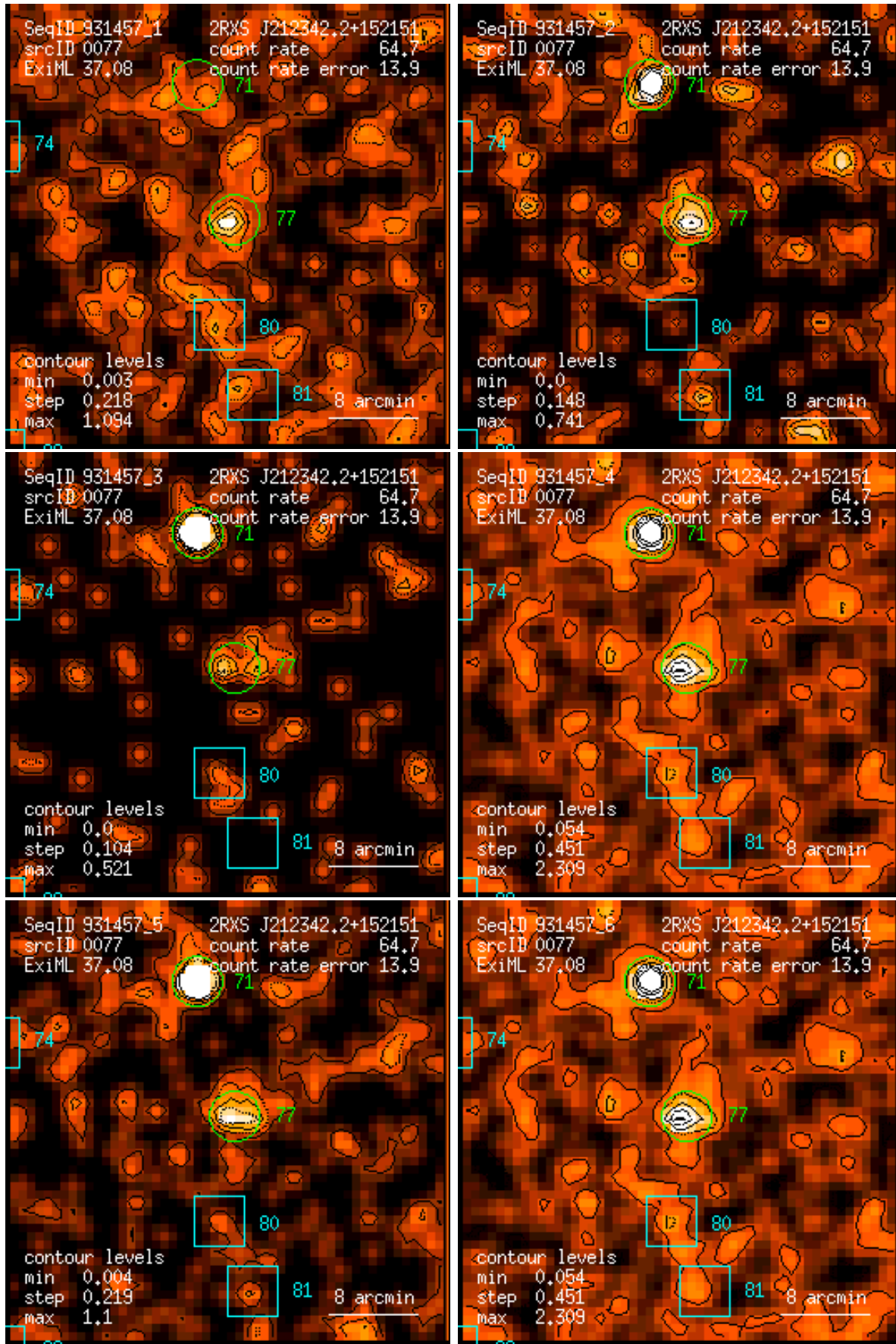
Figure 77: RASS 931457: detection 0077: band rate images, Gaussian filter: (1) PSPC channels 11 – 41, (2) 52 – 90, (3) 91 – 201, (4) 11 – 235, (5) 52 – 201, (6) 11 – 201. Broad band rates in counts/ks. Band rate contour levels in counts/ks/arcmin 2 .
