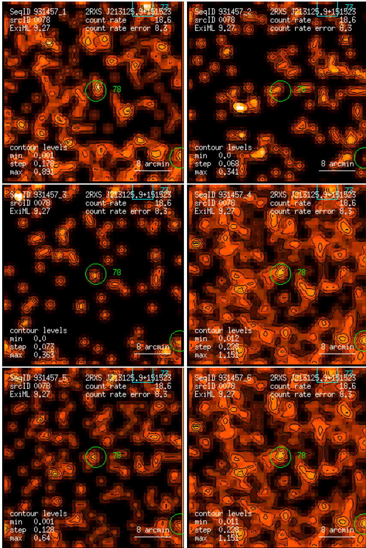
Figure 78: RASS 931457: detection 0078: band rate images, Gaussian filter: (1) PSPC channels 11 – 41, (2) 52 – 90, (3) 91 – 201, (4) 11 – 235, (5) 52 – 201, (6) 11 – 201. Broad band rates in counts/ks. Band rate contour levels in counts/ks/arcmin 2 .
