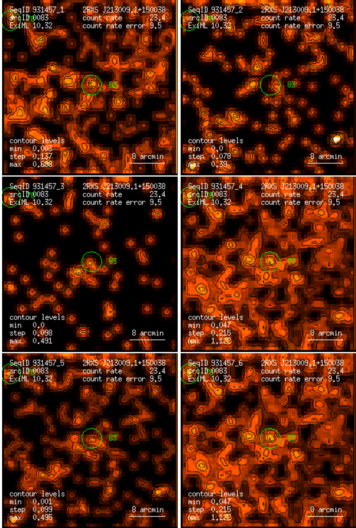
Figure 83: RASS 931457: detection 0083: band rate images, Gaussian filter: (1) PSPC channels 11 – 41, (2) 52 – 90, (3) 91 – 201, (4) 11 – 235, (5) 52 – 201, (6) 11 – 201. Broad band rates in counts/ks. Band rate contour levels in counts/ks/arcmin 2 .
