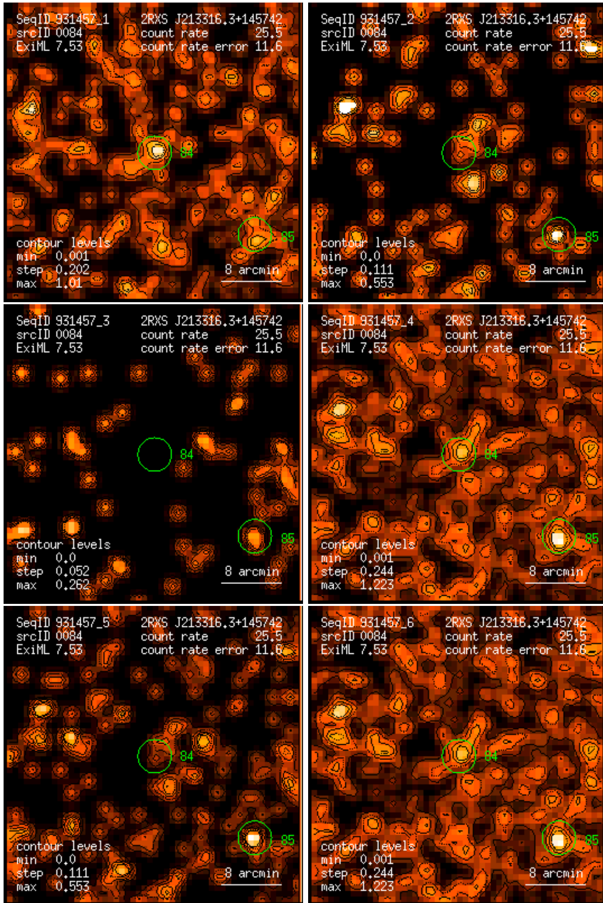
Figure 84: RASS 931457: detection 0084: band rate images, Gaussian filter: (1) PSPC channels 11 – 41, (2) 52 – 90, (3) 91 – 201, (4) 11 – 235, (5) 52 – 201, (6) 11 – 201. Broad band rates in counts/ks. Band rate contour levels in counts/ks/arcmin 2 .
