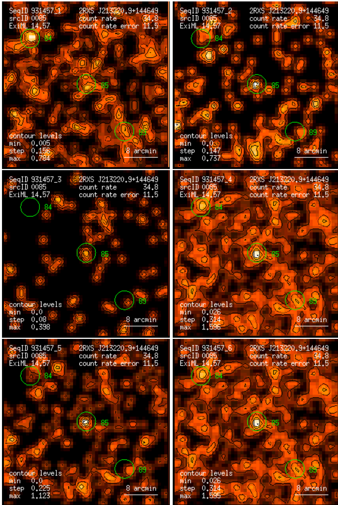
Figure 85: RASS 931457: detection 0085: band rate images, Gaussian filter: (1) PSPC channels 11 – 41, (2) 52 – 90, (3) 91 – 201, (4) 11 – 235, (5) 52 – 201, (6) 11 – 201. Broad band rates in counts/ks. Band rate contour levels in counts/ks/arcmin 2 .
