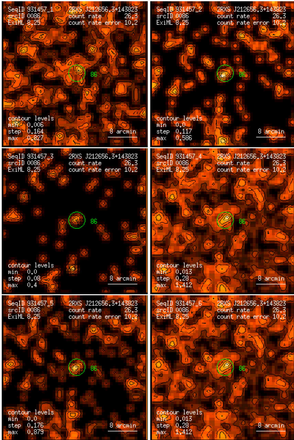
Figure 86: RASS 931457: detection 0086: band rate images, Gaussian filter: (1) PSPC channels 11 – 41, (2) 52 – 90, (3) 91 – 201, (4) 11 – 235, (5) 52 – 201, (6) 11 – 201. Broad band rates in counts/ks. Band rate contour levels in counts/ks/arcmin 2 .
