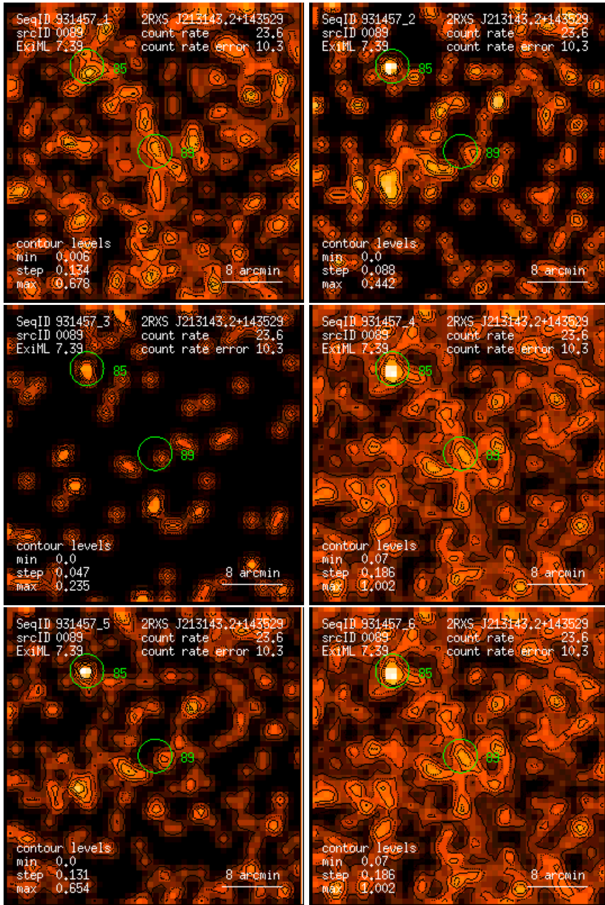
Figure 89: RASS 931457: detection 0089: band rate images, Gaussian filter: (1) PSPC channels 11 – 41, (2) 52 – 90, (3) 91 – 201, (4) 11 – 235, (5) 52 – 201, (6) 11 – 201. Broad band rates in counts/ks. Band rate contour levels in counts/ks/arcmin 2 .
