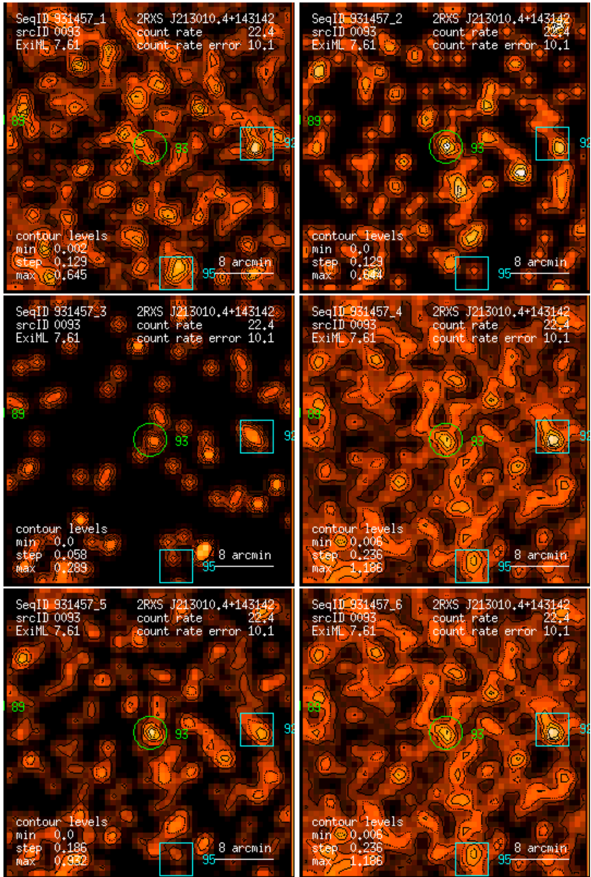
Figure 93: RASS 931457: detection 0093: band rate images, Gaussian filter: (1) PSPC channels 11 – 41, (2) 52 – 90, (3) 91 – 201, (4) 11 – 235, (5) 52 – 201, (6) 11 – 201. Broad band rates in counts/ks. Band rate contour levels in counts/ks/arcmin 2 .
