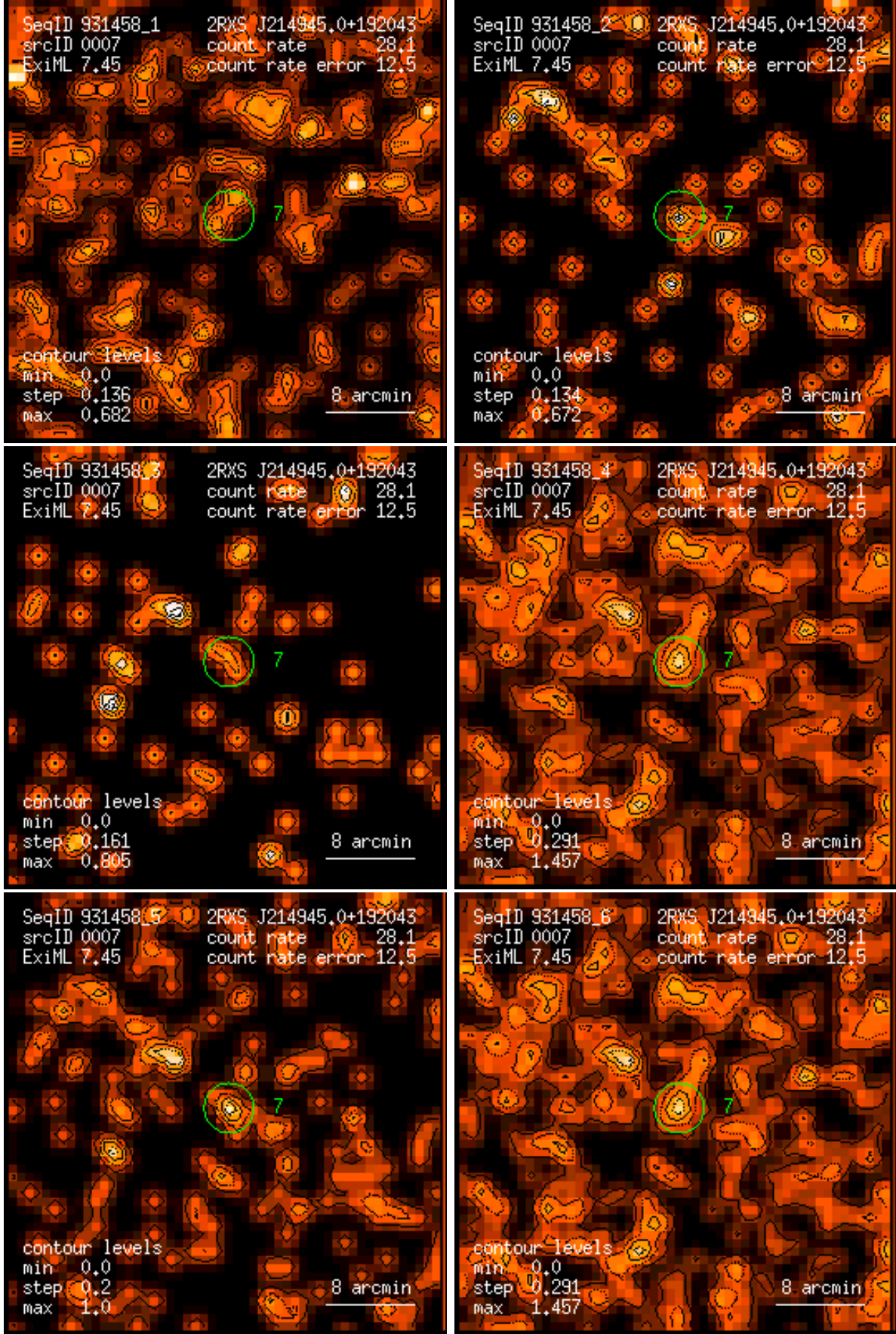
Figure 7: RASS 931458: detection 0007: band rate images, Gaussian filter: (1) PSPC channels 11 – 41, (2) 52 – 90, (3) 91 – 201, (4) 11 – 235, (5) 52 – 201, (6) 11 – 201. Broad band rates in counts/ks. Band rate contour levels in counts/ks/arcmin 2 .
