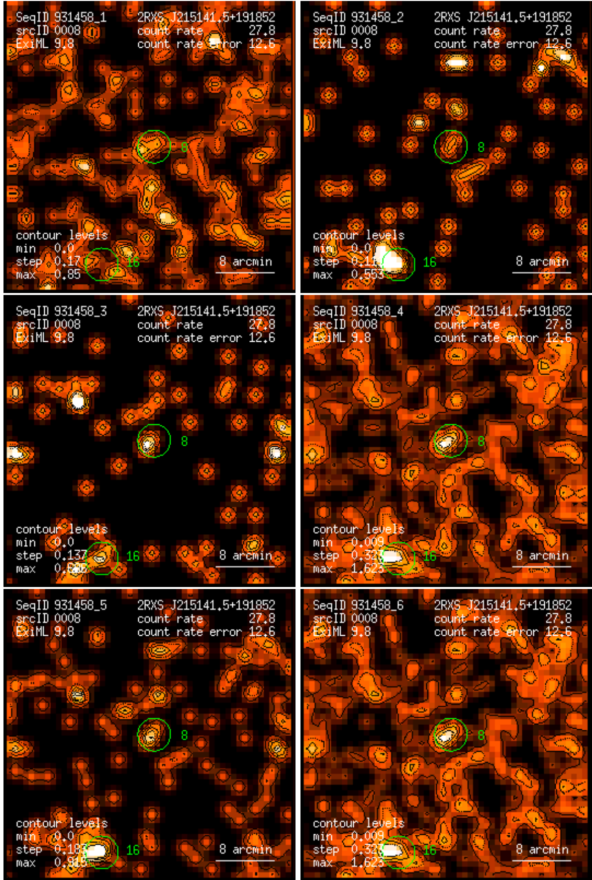
Figure 8: RASS 931458: detection 0008: band rate images, Gaussian filter: (1) PSPC channels 11 – 41, (2) 52 – 90, (3) 91 – 201, (4) 11 – 235, (5) 52 – 201, (6) 11 – 201. Broad band rates in counts/ks. Band rate contour levels in counts/ks/arcmin 2 .
