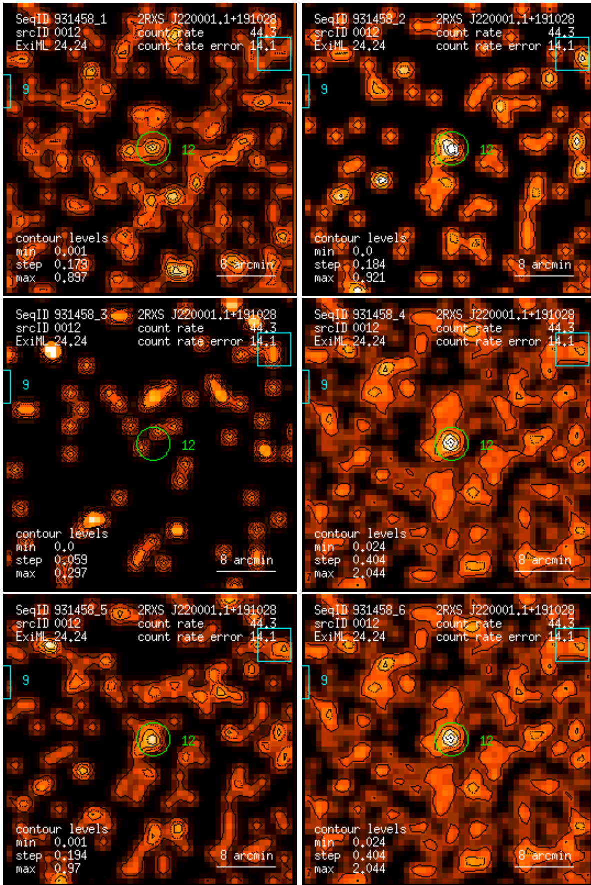
Figure 12: RASS 931458: detection 0012: band rate images, Gaussian filter: (1) PSPC channels 11 – 41, (2) 52 – 90, (3) 91 – 201, (4) 11 – 235, (5) 52 – 201, (6) 11 – 201. Broad band rates in counts/ks. Band rate contour levels in counts/ks/arcmin 2 .
