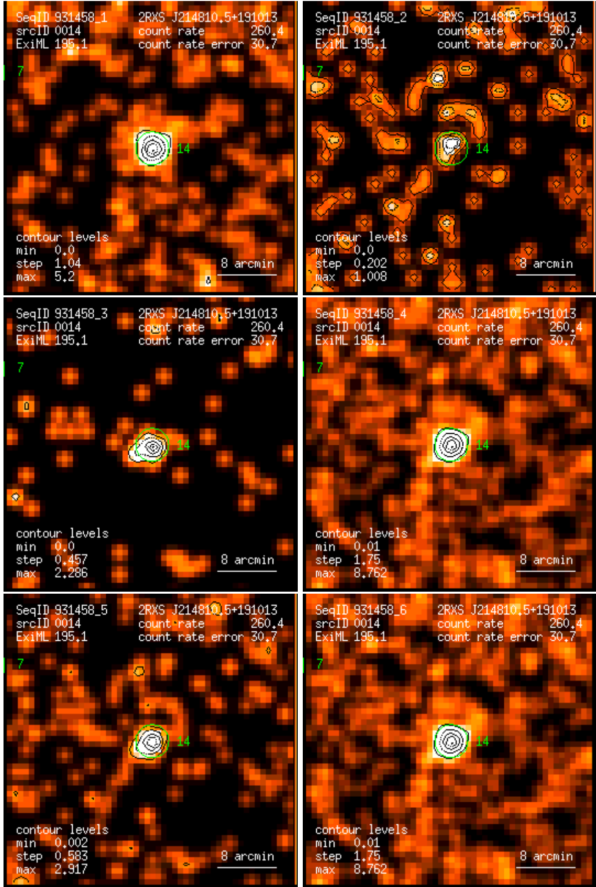
Figure 14: RASS 931458: detection 0014: band rate images, Gaussian filter: (1) PSPC channels 11 – 41, (2) 52 – 90, (3) 91 – 201, (4) 11 – 235, (5) 52 – 201, (6) 11 – 201. Broad band rates in counts/ks. Band rate contour levels in counts/ks/arcmin 2 .
