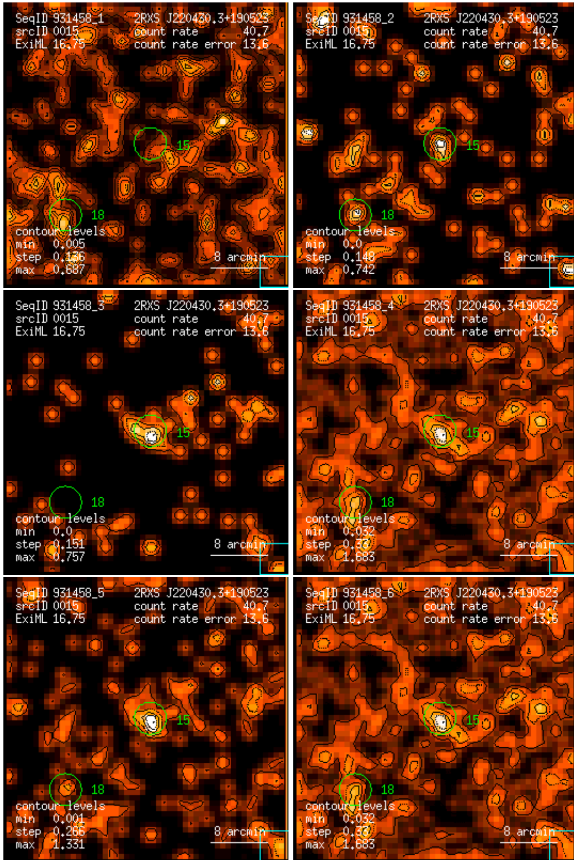
Figure 15: RASS 931458: detection 0015: band rate images, Gaussian filter: (1) PSPC channels 11 – 41, (2) 52 – 90, (3) 91 – 201, (4) 11 – 235, (5) 52 – 201, (6) 11 – 201. Broad band rates in counts/ks. Band rate contour levels in counts/ks/arcmin 2 .
