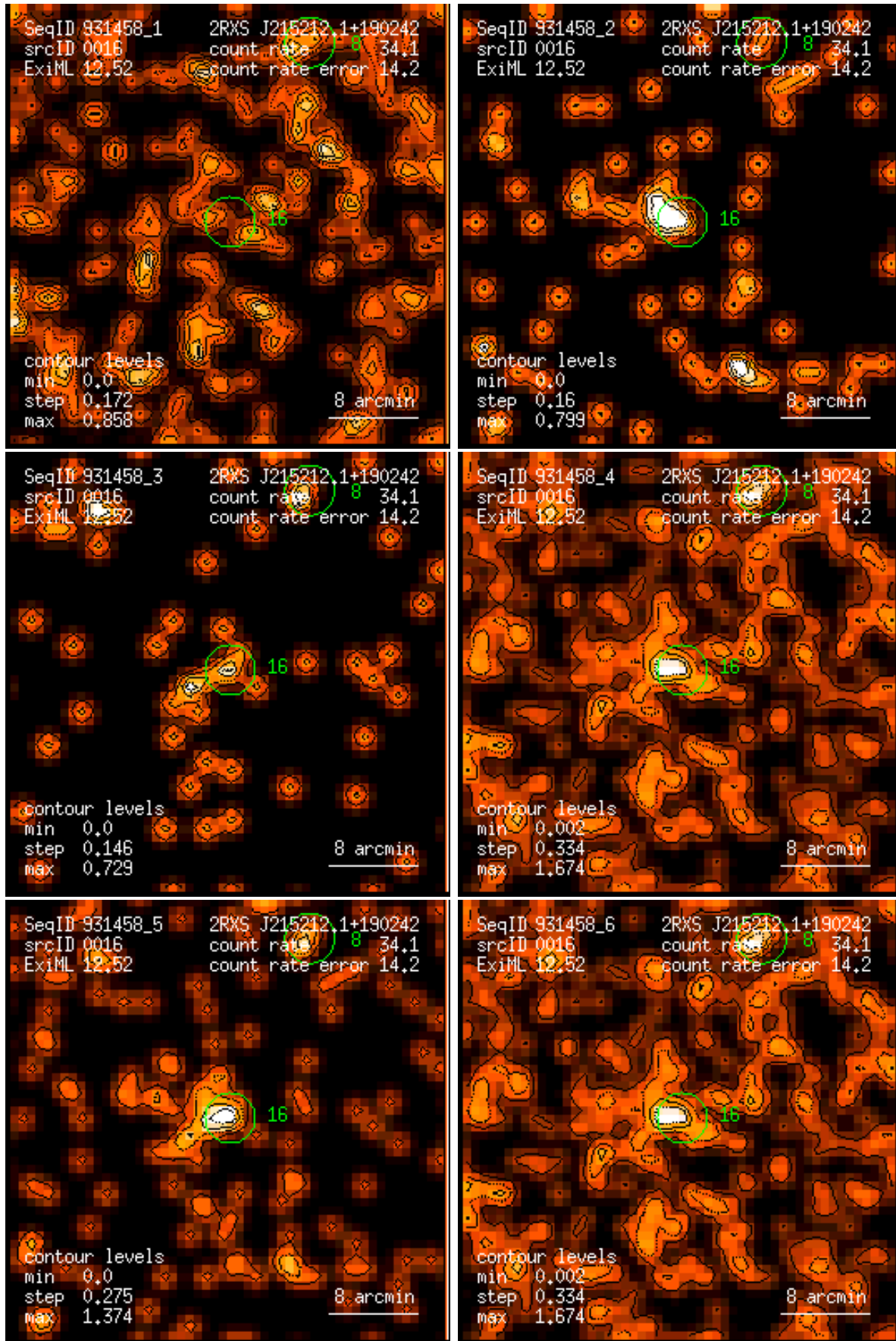
Figure 16: RASS 931458: detection 0016: band rate images, Gaussian filter: (1) PSPC channels 11 – 41, (2) 52 – 90, (3) 91 – 201, (4) 11 – 235, (5) 52 – 201, (6) 11 – 201. Broad band rates in counts/ks. Band rate contour levels in counts/ks/arcmin 2 .
