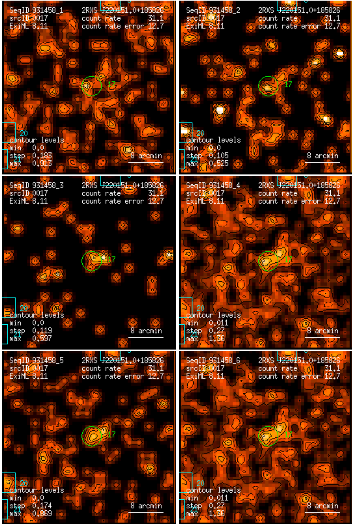
Figure 17: RASS 931458: detection 0017: band rate images, Gaussian filter: (1) PSPC channels 11 – 41, (2) 52 – 90, (3) 91 – 201, (4) 11 – 235, (5) 52 – 201, (6) 11 – 201. Broad band rates in counts/ks. Band rate contour levels in counts/ks/arcmin 2 .
