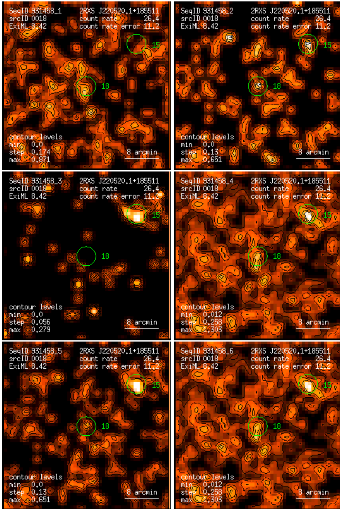
Figure 18: RASS 931458: detection 0018: band rate images, Gaussian filter: (1) PSPC channels 11 – 41, (2) 52 – 90, (3) 91 – 201, (4) 11 – 235, (5) 52 – 201, (6) 11 – 201. Broad band rates in counts/ks. Band rate contour levels in counts/ks/arcmin 2 .
