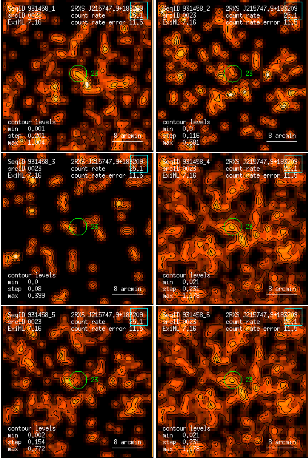
Figure 23: RASS 931458: detection 0023: band rate images, Gaussian filter: (1) PSPC channels 11 – 41, (2) 52 – 90, (3) 91 – 201, (4) 11 – 235, (5) 52 – 201, (6) 11 – 201. Broad band rates in counts/ks. Band rate contour levels in counts/ks/arcmin 2 .
