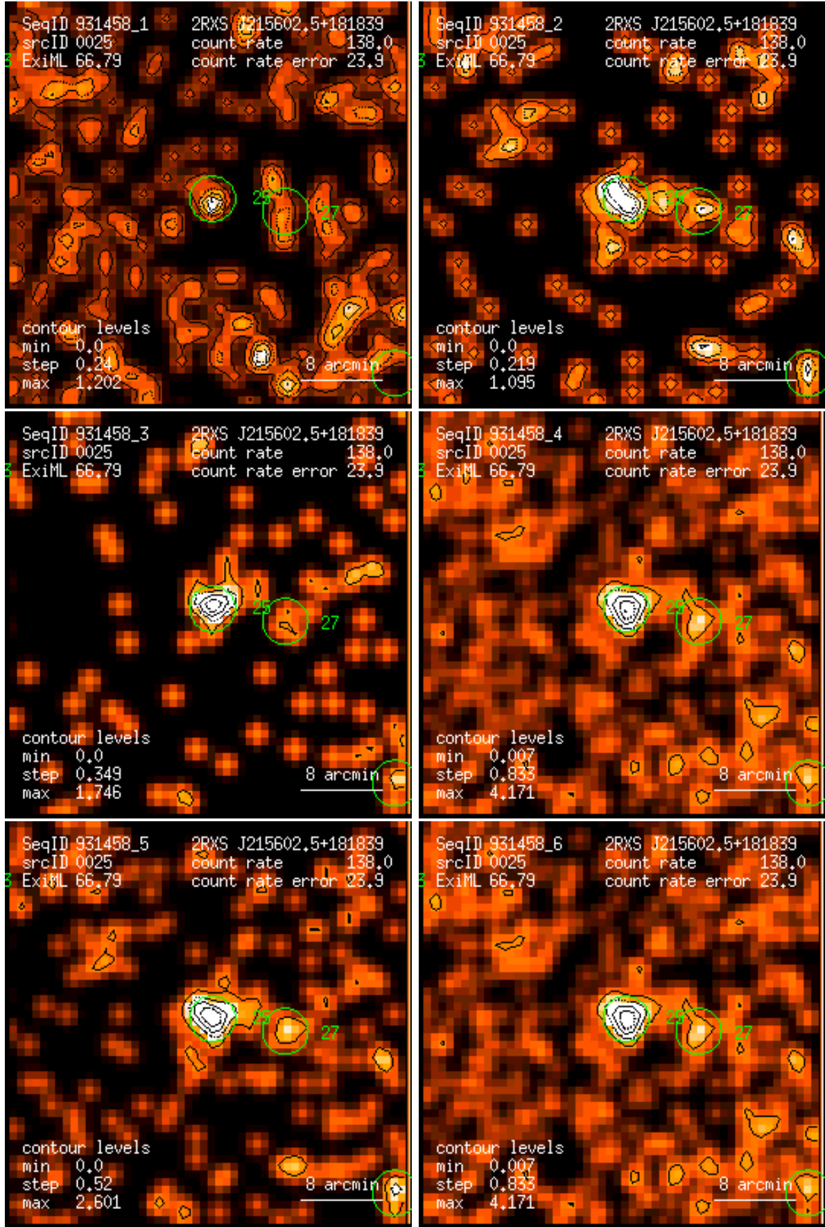
Figure 25: RASS 931458: detection 0025: band rate images, Gaussian filter: (1) PSPC channels 11 – 41, (2) 52 – 90, (3) 91 – 201, (4) 11 – 235, (5) 52 – 201, (6) 11 – 201. Broad band rates in counts/ks. Band rate contour levels in counts/ks/arcmin 2 .
