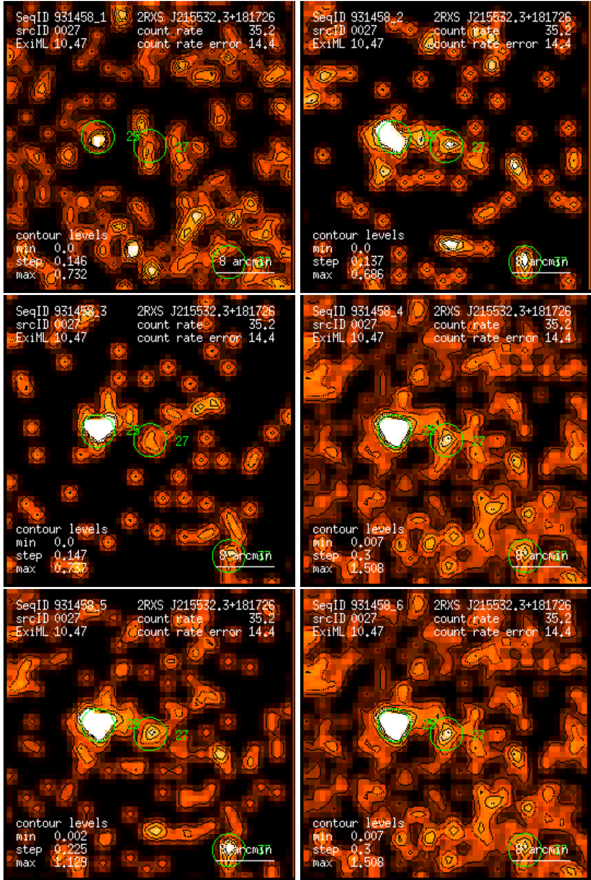
Figure 27: RASS 931458: detection 0027: band rate images, Gaussian filter: (1) PSPC channels 11 – 41, (2) 52 – 90, (3) 91 – 201, (4) 11 – 235, (5) 52 – 201, (6) 11 – 201. Broad band rates in counts/ks. Band rate contour levels in counts/ks/arcmin 2 .
