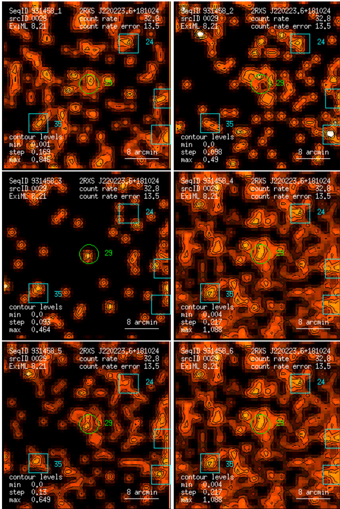
Figure 29: RASS 931458: detection 0029: band rate images, Gaussian filter: (1) PSPC channels 11 – 41, (2) 52 – 90, (3) 91 – 201, (4) 11 – 235, (5) 52 – 201, (6) 11 – 201. Broad band rates in counts/ks. Band rate contour levels in counts/ks/arcmin 2 .
