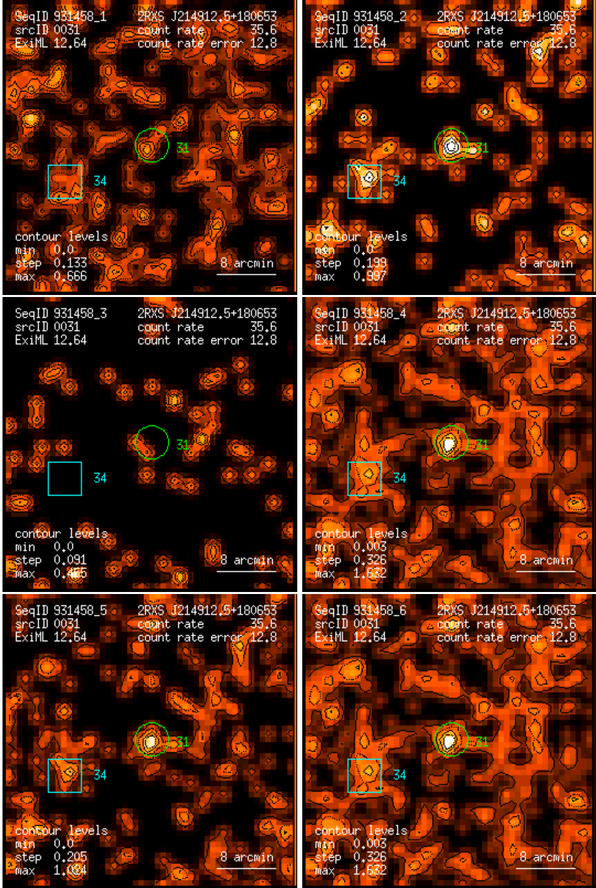
Figure 31: RASS 931458: detection 0031: band rate images, Gaussian filter: (1) PSPC channels 11 – 41, (2) 52 – 90, (3) 91 – 201, (4) 11 – 235, (5) 52 – 201, (6) 11 – 201. Broad band rates in counts/ks. Band rate contour levels in counts/ks/arcmin 2 .
