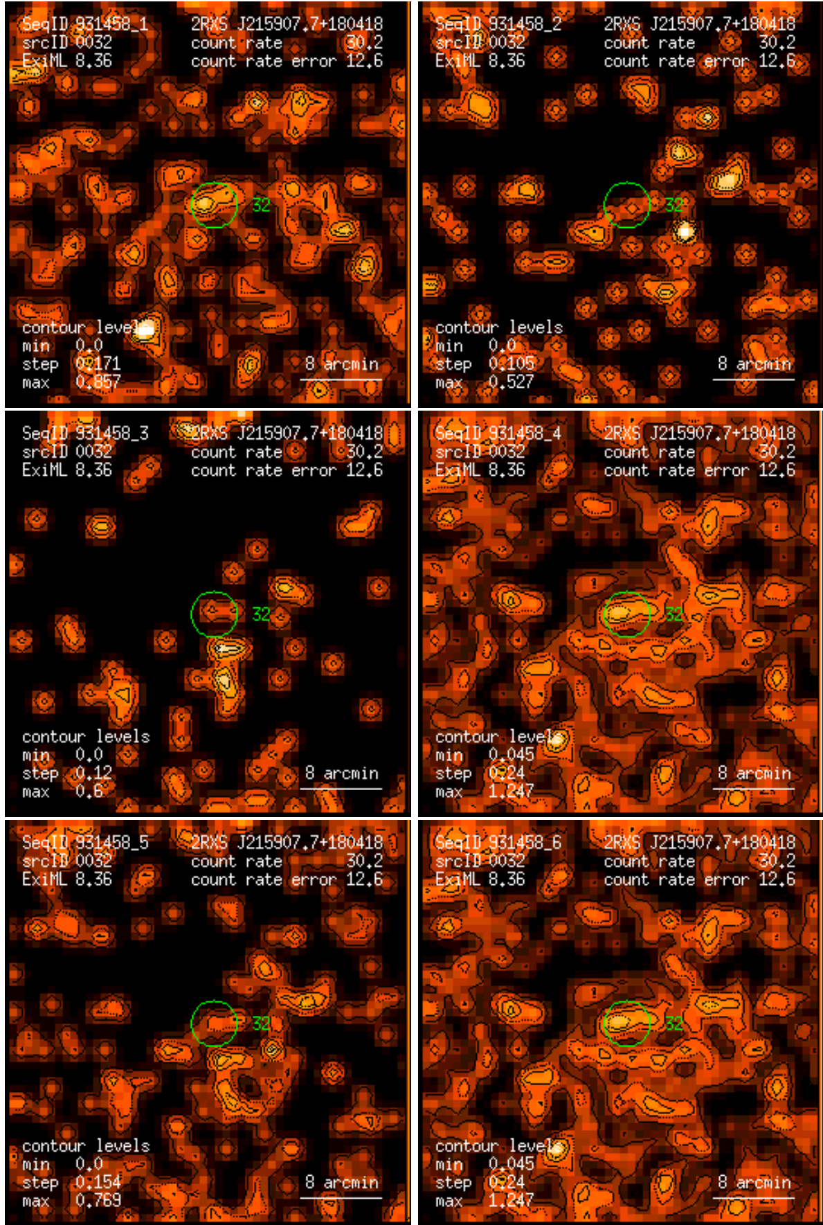
Figure 32: RASS 931458: detection 0032: band rate images, Gaussian filter: (1) PSPC channels 11 – 41, (2) 52 – 90, (3) 91 – 201, (4) 11 – 235, (5) 52 – 201, (6) 11 – 201. Broad band rates in counts/ks. Band rate contour levels in counts/ks/arcmin 2 .
