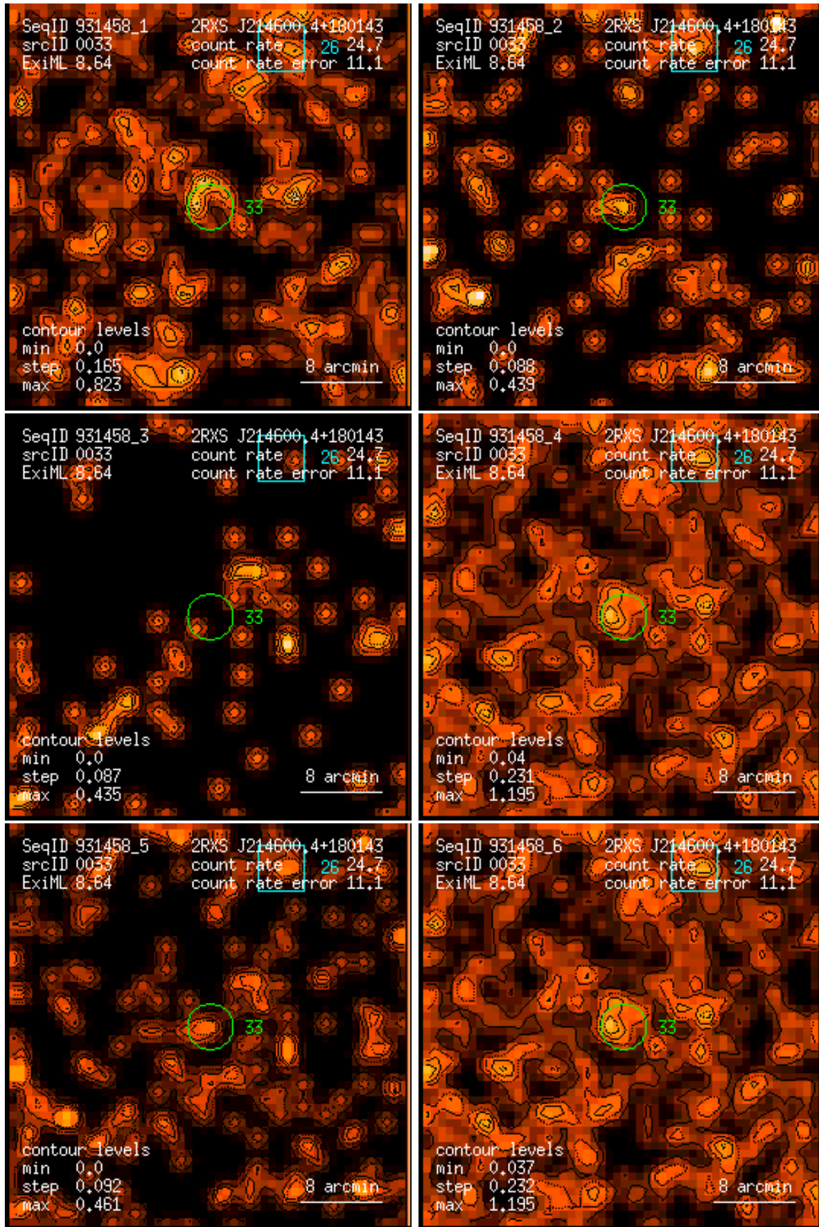
Figure 33: RASS 931458: detection 0033: band rate images, Gaussian filter: (1) PSPC channels 11 – 41, (2) 52 – 90, (3) 91 – 201, (4) 11 – 235, (5) 52 – 201, (6) 11 – 201. Broad band rates in counts/ks. Band rate contour levels in counts/ks/arcmin 2 .
