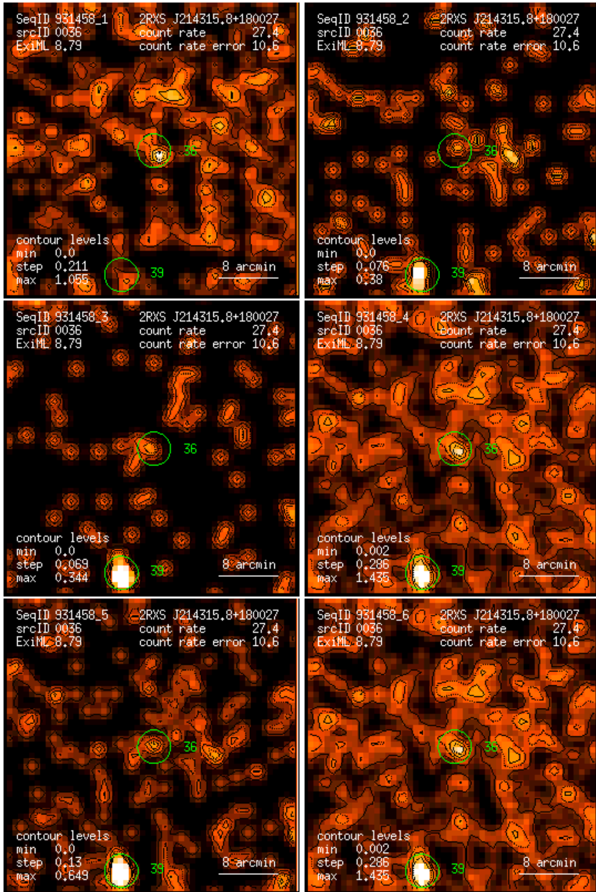
Figure 36: RASS 931458: detection 0036: band rate images, Gaussian filter: (1) PSPC channels 11 – 41, (2) 52 – 90, (3) 91 – 201, (4) 11 – 235, (5) 52 – 201, (6) 11 – 201. Broad band rates in counts/ks. Band rate contour levels in counts/ks/arcmin 2 .
