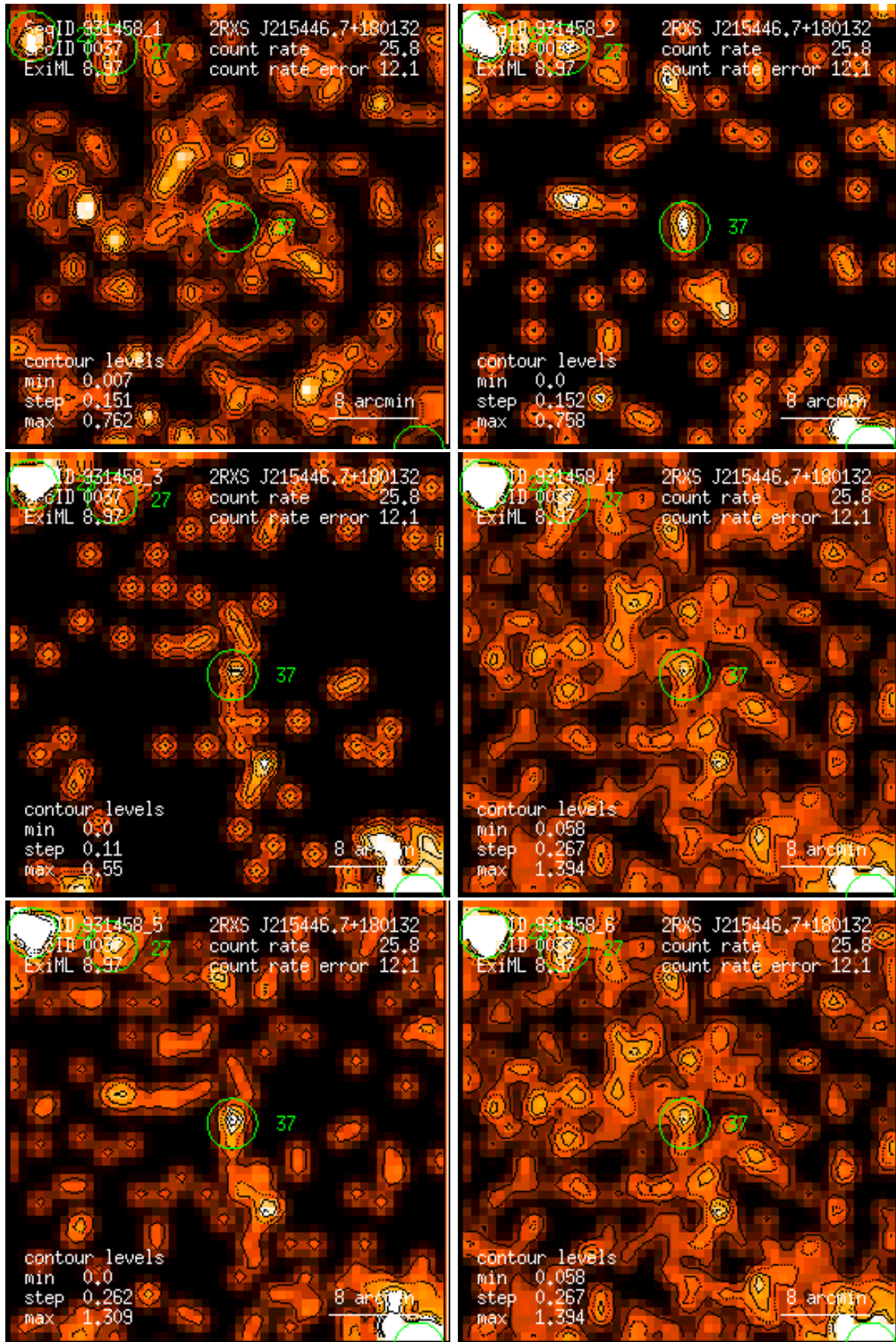
Figure 37: RASS 931458: detection 0037: band rate images, Gaussian filter: (1) PSPC channels 11 – 41, (2) 52 – 90, (3) 91 – 201, (4) 11 – 235, (5) 52 – 201, (6) 11 – 201. Broad band rates in counts/ks. Band rate contour levels in counts/ks/arcmin 2 .
