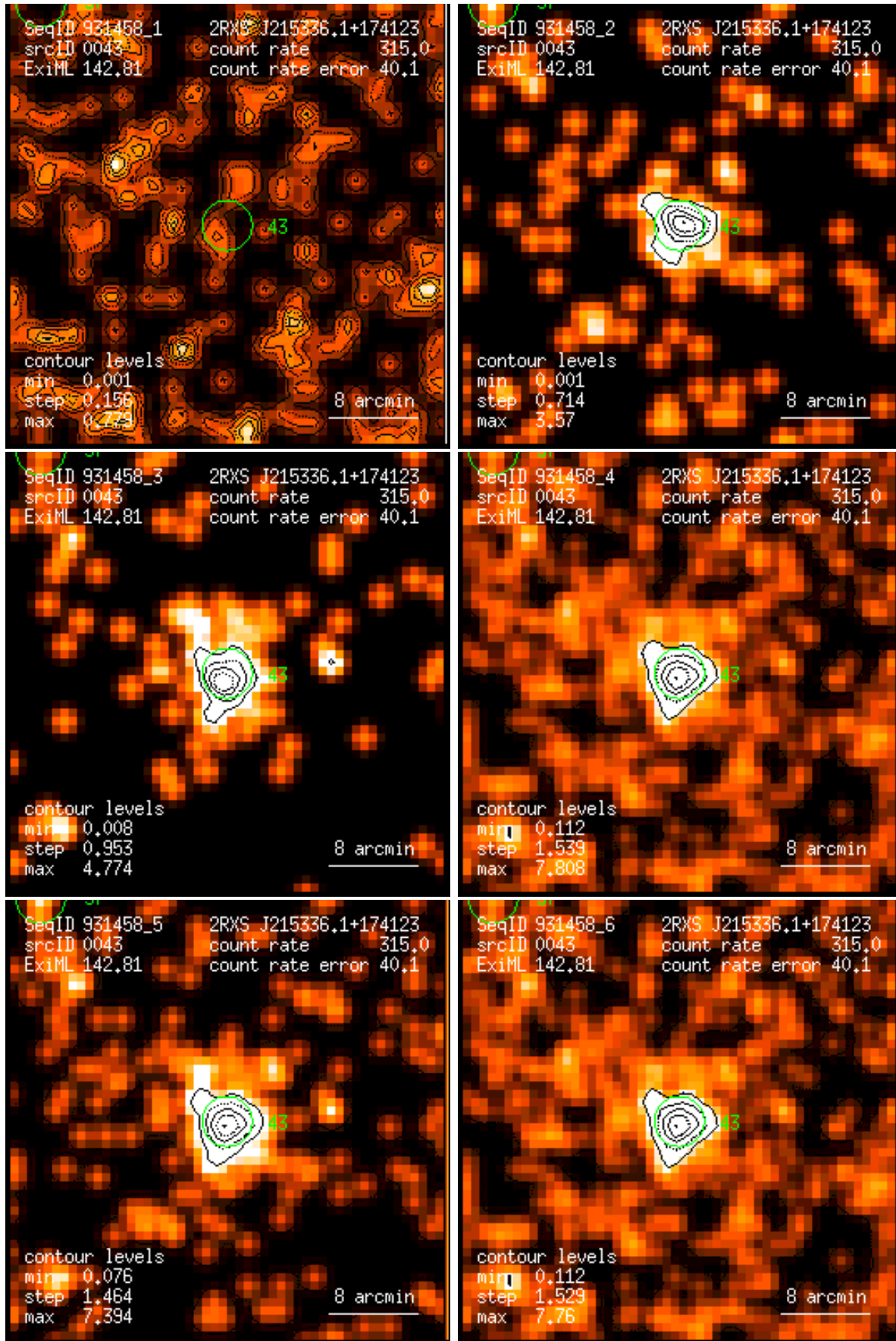
Figure 43: RASS 931458: detection 0043: band rate images, Gaussian filter: (1) PSPC channels 11 – 41, (2) 52 – 90, (3) 91 – 201, (4) 11 – 235, (5) 52 – 201, (6) 11 – 201. Broad band rates in counts/ks. Band rate contour levels in counts/ks/arcmin 2 .
