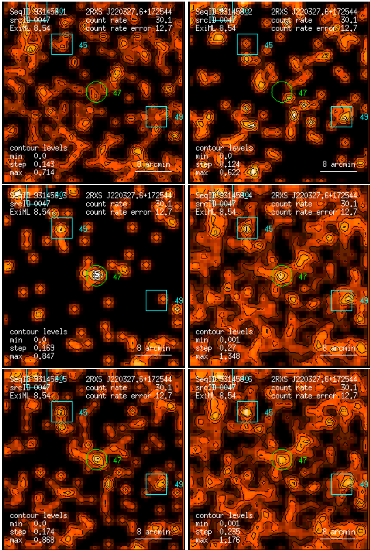
Figure 47: RASS 931458: detection 0047: band rate images, Gaussian filter: (1) PSPC channels 11 – 41, (2) 52 – 90, (3) 91 – 201, (4) 11 – 235, (5) 52 – 201, (6) 11 – 201. Broad band rates in counts/ks. Band rate contour levels in counts/ks/arcmin 2 .
