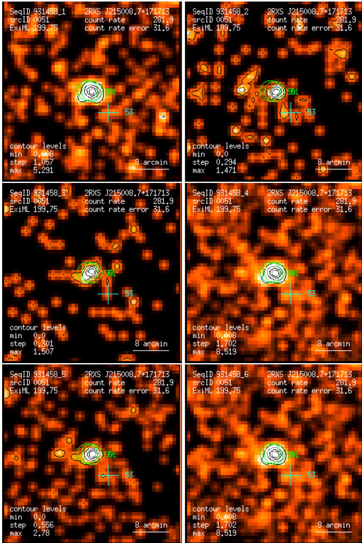
Figure 51: RASS 931458: detection 0051: band rate images, Gaussian filter: (1) PSPC channels 11 – 41, (2) 52 – 90, (3) 91 – 201, (4) 11 – 235, (5) 52 – 201, (6) 11 – 201. Broad band rates in counts/ks. Band rate contour levels in counts/ks/arcmin 2 .
