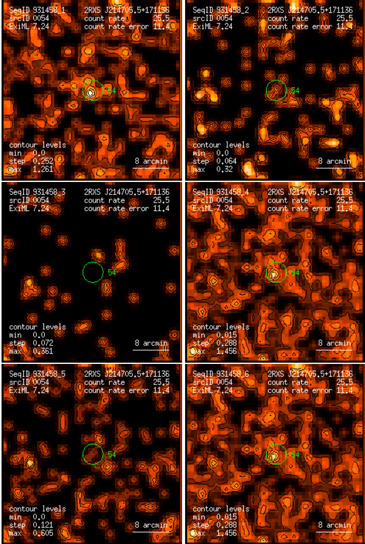
Figure 54: RASS 931458: detection 0054: band rate images, Gaussian filter: (1) PSPC channels 11 – 41, (2) 52 – 90, (3) 91 – 201, (4) 11 – 235, (5) 52 – 201, (6) 11 – 201. Broad band rates in counts/ks. Band rate contour levels in counts/ks/arcmin 2 .
