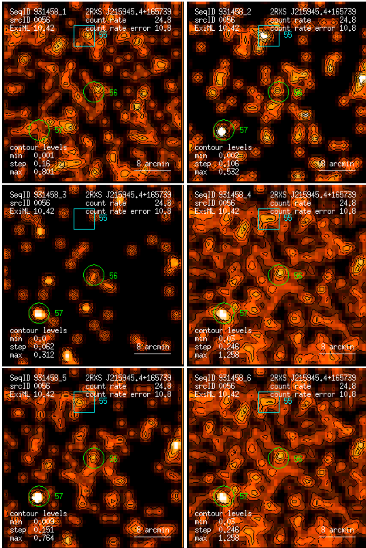
Figure 56: RASS 931458: detection 0056: band rate images, Gaussian filter: (1) PSPC channels 11 – 41, (2) 52 – 90, (3) 91 – 201, (4) 11 – 235, (5) 52 – 201, (6) 11 – 201. Broad band rates in counts/ks. Band rate contour levels in counts/ks/arcmin 2 .
