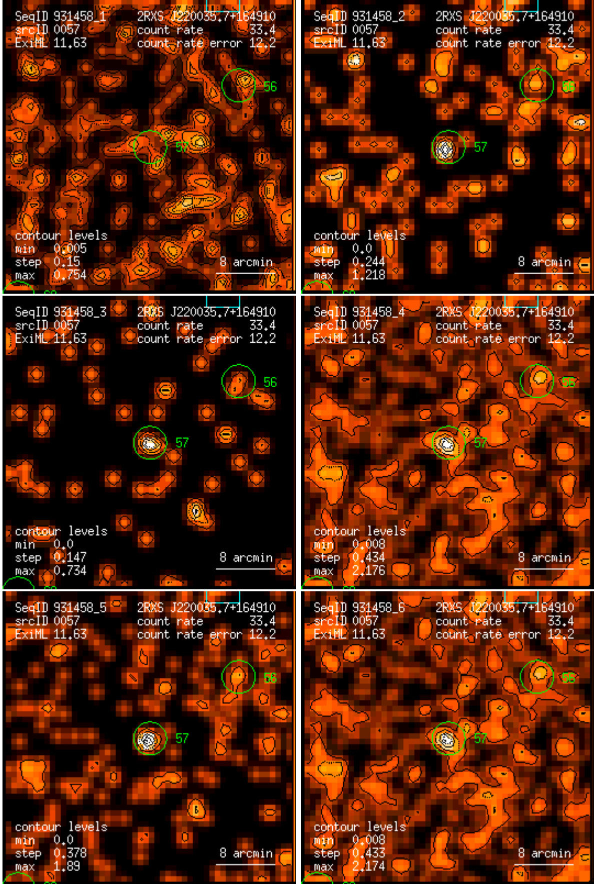
Figure 57: RASS 931458: detection 0057: band rate images, Gaussian filter: (1) PSPC channels 11 – 41, (2) 52 – 90, (3) 91 – 201, (4) 11 – 235, (5) 52 – 201, (6) 11 – 201. Broad band rates in counts/ks. Band rate contour levels in counts/ks/arcmin 2 .
