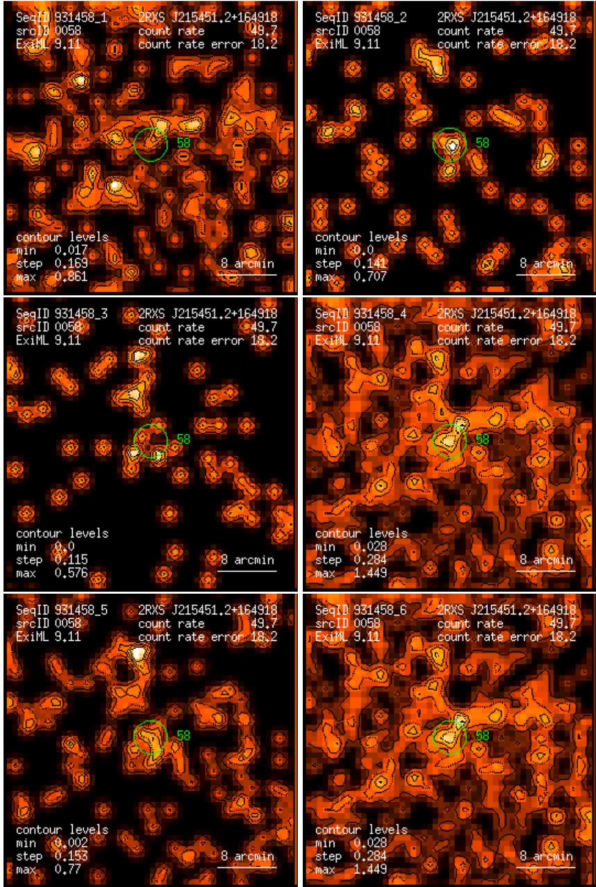
Figure 58: RASS 931458: detection 0058: band rate images, Gaussian filter: (1) PSPC channels 11 – 41, (2) 52 – 90, (3) 91 – 201, (4) 11 – 235, (5) 52 – 201, (6) 11 – 201. Broad band rates in counts/ks. Band rate contour levels in counts/ks/arcmin 2 .
