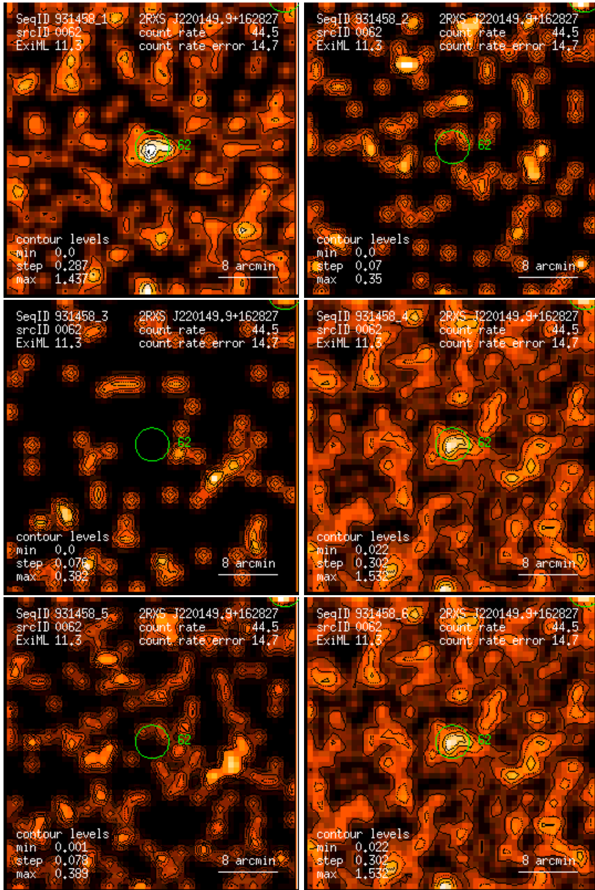
Figure 62: RASS 931458: detection 0062: band rate images, Gaussian filter: (1) PSPC channels 11 – 41, (2) 52 – 90, (3) 91 – 201, (4) 11 – 235, (5) 52 – 201, (6) 11 – 201. Broad band rates in counts/ks. Band rate contour levels in counts/ks/arcmin 2 .
