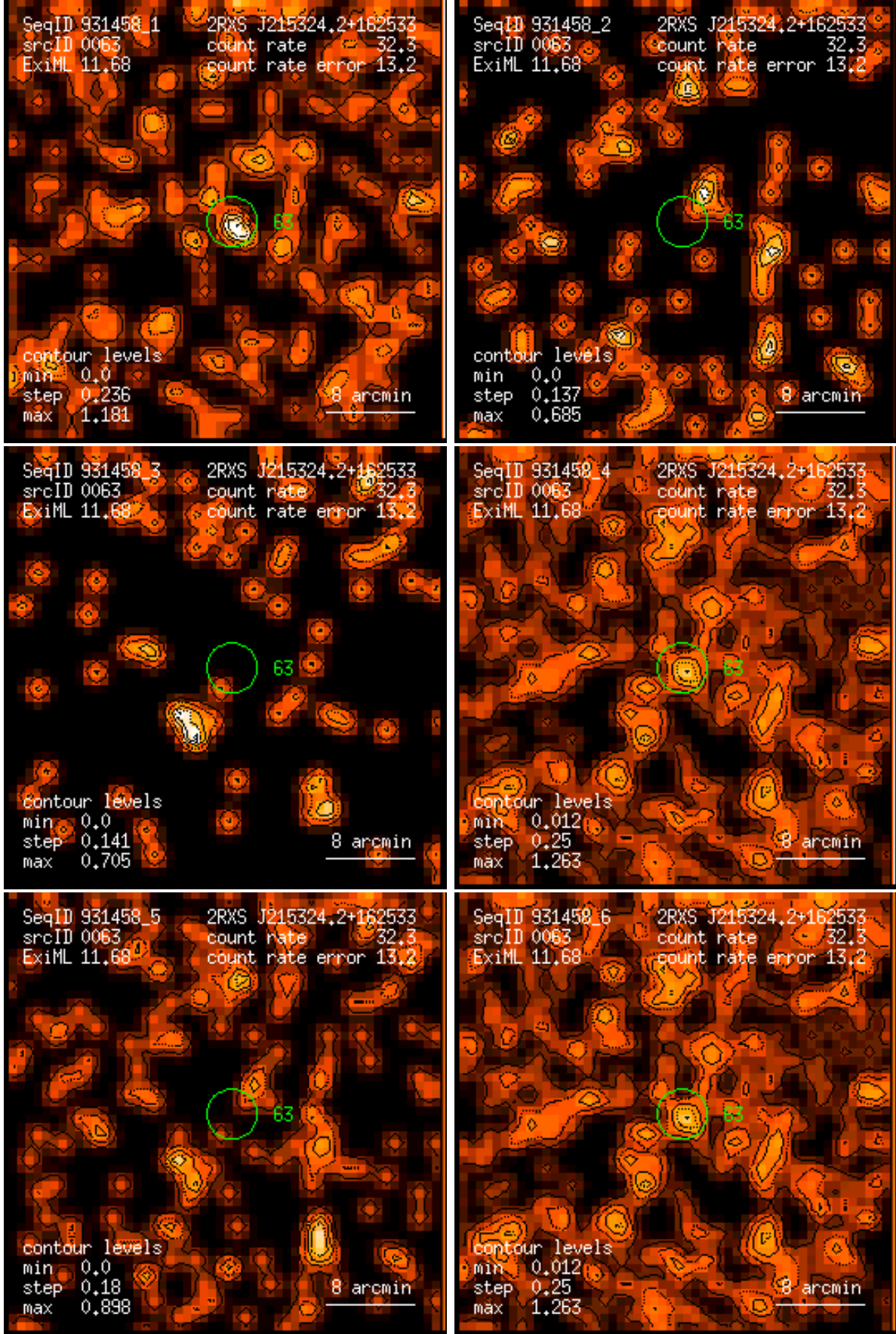
Figure 63: RASS 931458: detection 0063: band rate images, Gaussian filter: (1) PSPC channels 11 – 41, (2) 52 – 90, (3) 91 – 201, (4) 11 – 235, (5) 52 – 201, (6) 11 – 201. Broad band rates in counts/ks. Band rate contour levels in counts/ks/arcmin 2 .
