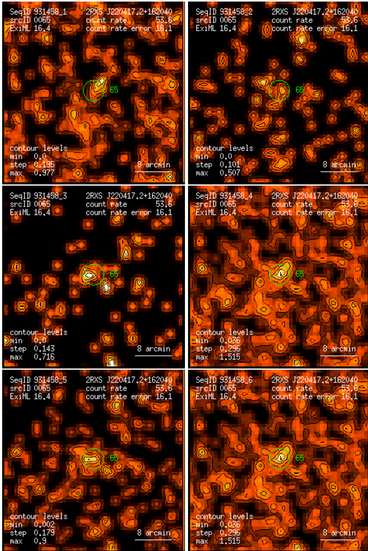
Figure 65: RASS 931458: detection 0065: band rate images, Gaussian filter: (1) PSPC channels 11 – 41, (2) 52 – 90, (3) 91 – 201, (4) 11 – 235, (5) 52 – 201, (6) 11 – 201. Broad band rates in counts/ks. Band rate contour levels in counts/ks/arcmin 2 .
