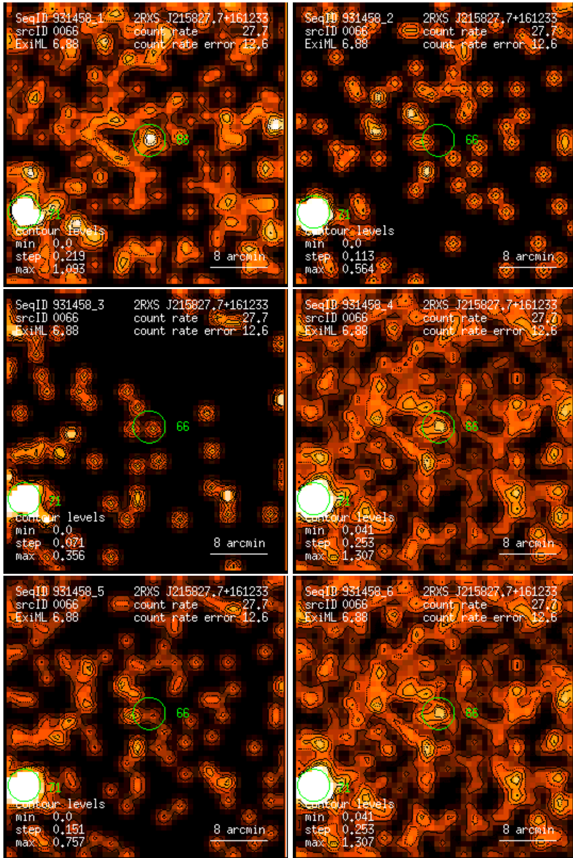
Figure 66: RASS 931458: detection 0066: band rate images, Gaussian filter: (1) PSPC channels 11 – 41, (2) 52 – 90, (3) 91 – 201, (4) 11 – 235, (5) 52 – 201, (6) 11 – 201. Broad band rates in counts/ks. Band rate contour levels in counts/ks/arcmin 2 .
