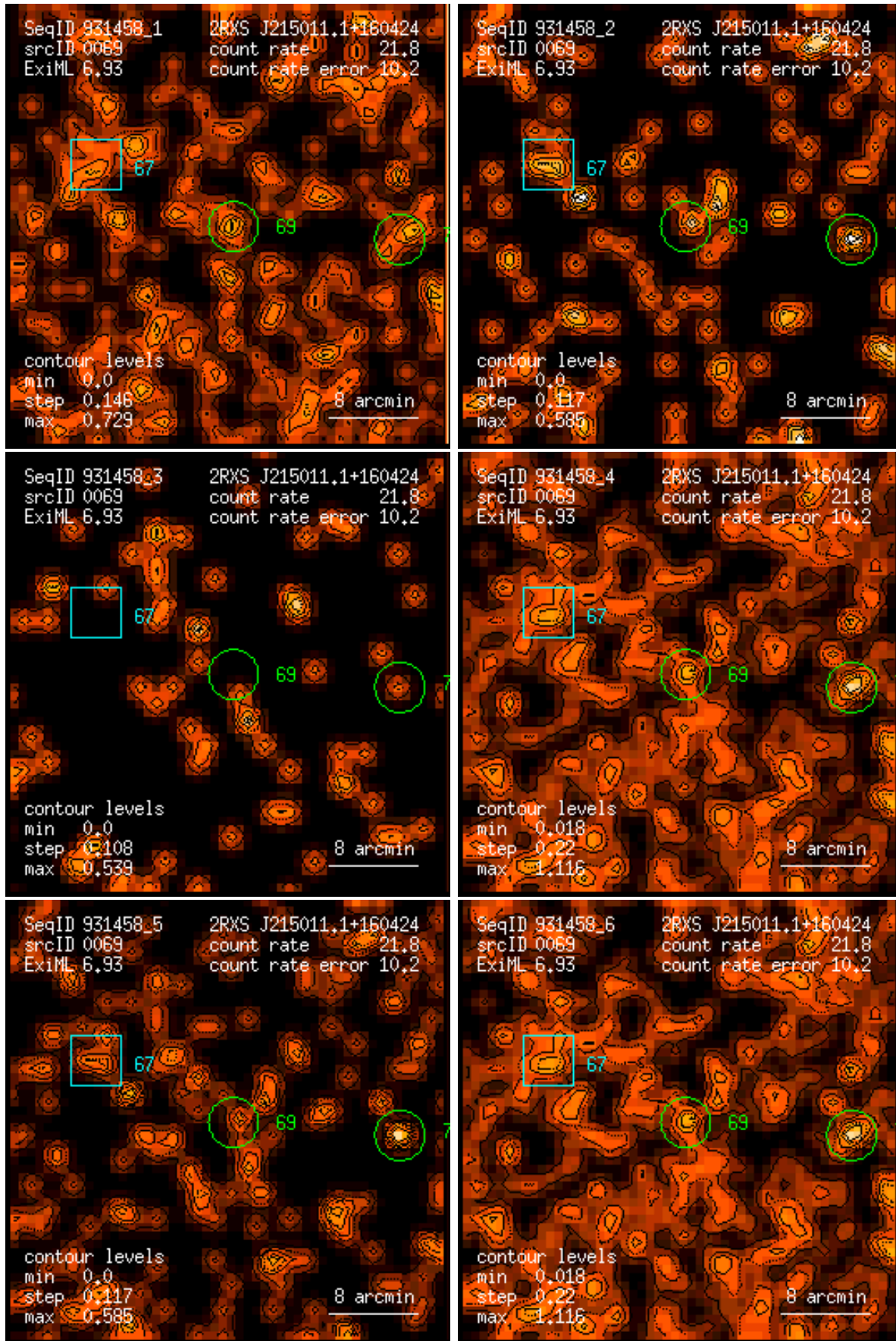
Figure 69: RASS 931458: detection 0069: band rate images, Gaussian filter: (1) PSPC channels 11 – 41, (2) 52 – 90, (3) 91 – 201, (4) 11 – 235, (5) 52 – 201, (6) 11 – 201. Broad band rates in counts/ks. Band rate contour levels in counts/ks/arcmin 2 .
