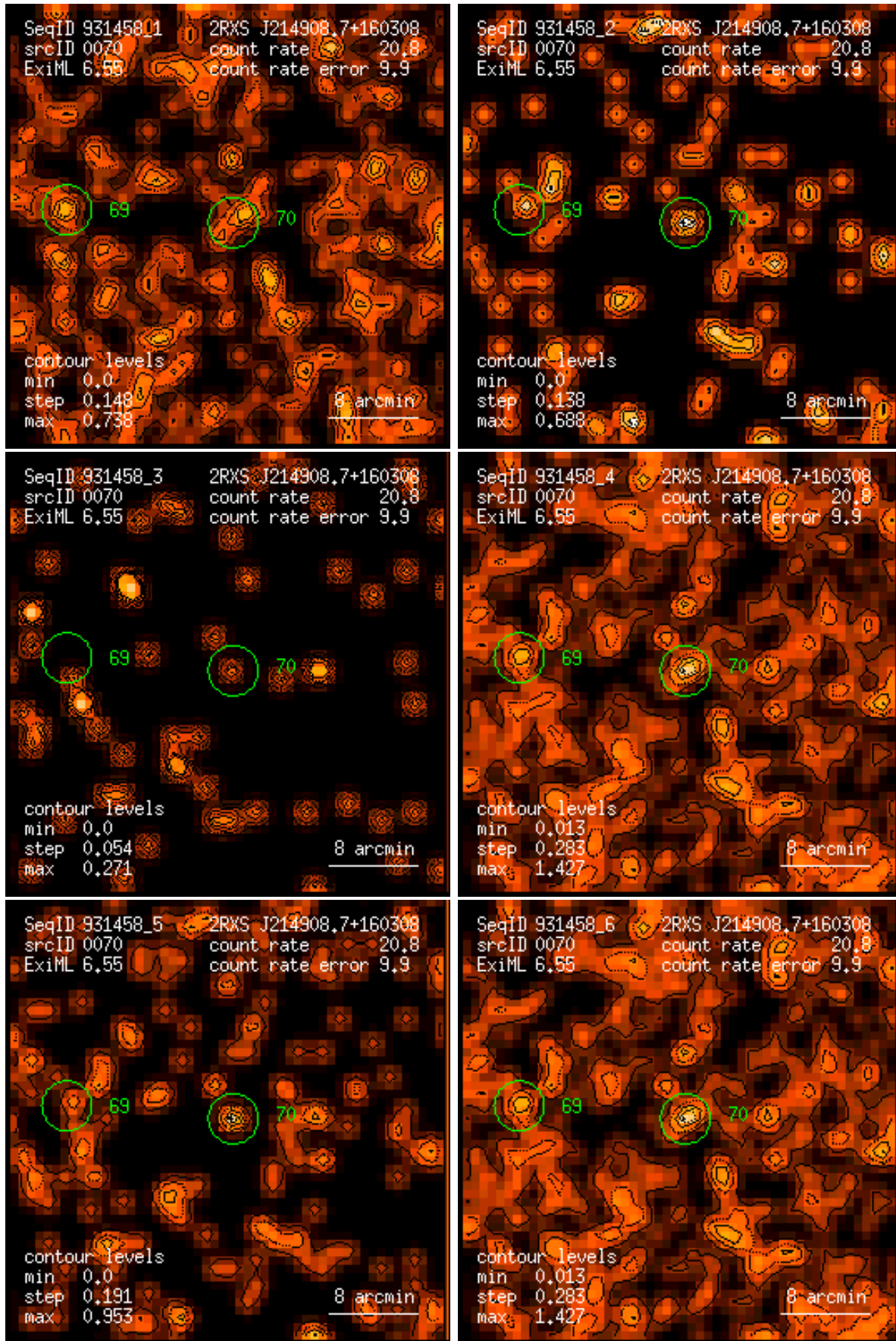
Figure 70: RASS 931458: detection 0070: band rate images, Gaussian filter: (1) PSPC channels 11 – 41, (2) 52 – 90, (3) 91 – 201, (4) 11 – 235, (5) 52 – 201, (6) 11 – 201. Broad band rates in counts/ks. Band rate contour levels in counts/ks/arcmin 2 .
