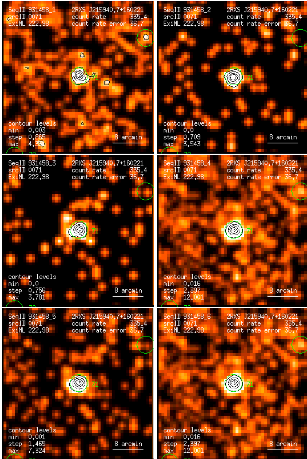
Figure 71: RASS 931458: detection 0071: band rate images, Gaussian filter: (1) PSPC channels 11 – 41, (2) 52 – 90, (3) 91 – 201, (4) 11 – 235, (5) 52 – 201, (6) 11 – 201. Broad band rates in counts/ks. Band rate contour levels in counts/ks/arcmin 2 .
