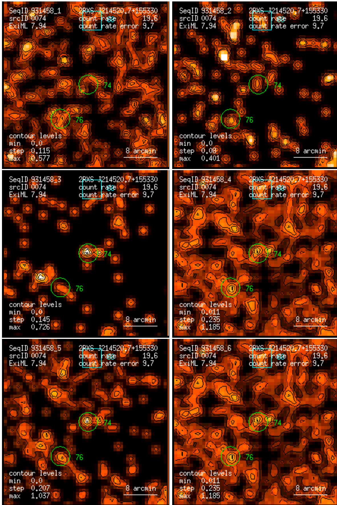
Figure 74: RASS 931458: detection 0074: band rate images, Gaussian filter: (1) PSPC channels 11 – 41, (2) 52 – 90, (3) 91 – 201, (4) 11 – 235, (5) 52 – 201, (6) 11 – 201. Broad band rates in counts/ks. Band rate contour levels in counts/ks/arcmin 2 .
