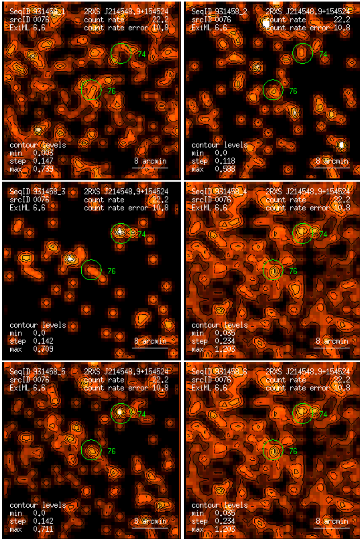
Figure 76: RASS 931458: detection 0076: band rate images, Gaussian filter: (1) PSPC channels 11 – 41, (2) 52 – 90, (3) 91 – 201, (4) 11 – 235, (5) 52 – 201, (6) 11 – 201. Broad band rates in counts/ks. Band rate contour levels in counts/ks/arcmin 2 .
