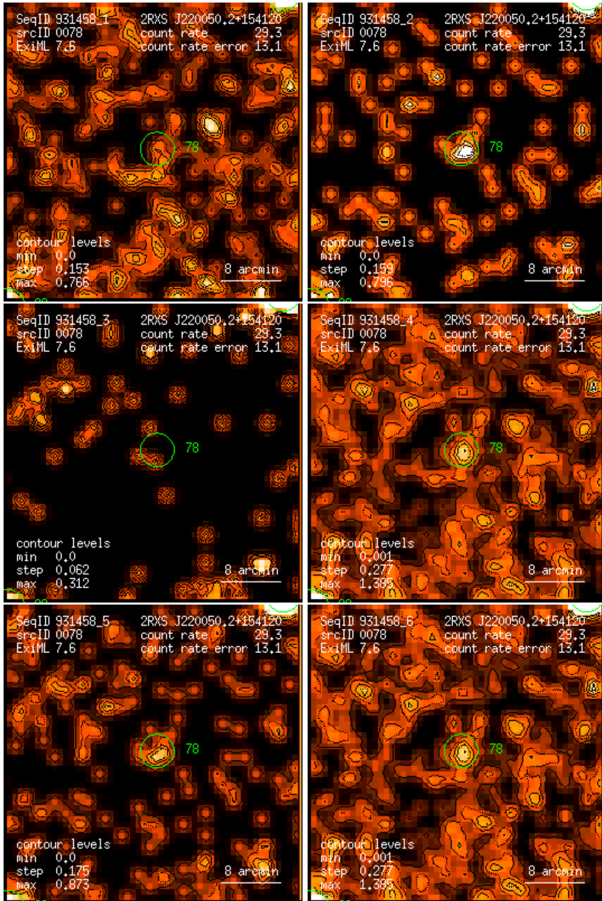
Figure 78: RASS 931458: detection 0078: band rate images, Gaussian filter: (1) PSPC channels 11 – 41, (2) 52 – 90, (3) 91 – 201, (4) 11 – 235, (5) 52 – 201, (6) 11 – 201. Broad band rates in counts/ks. Band rate contour levels in counts/ks/arcmin 2 .
