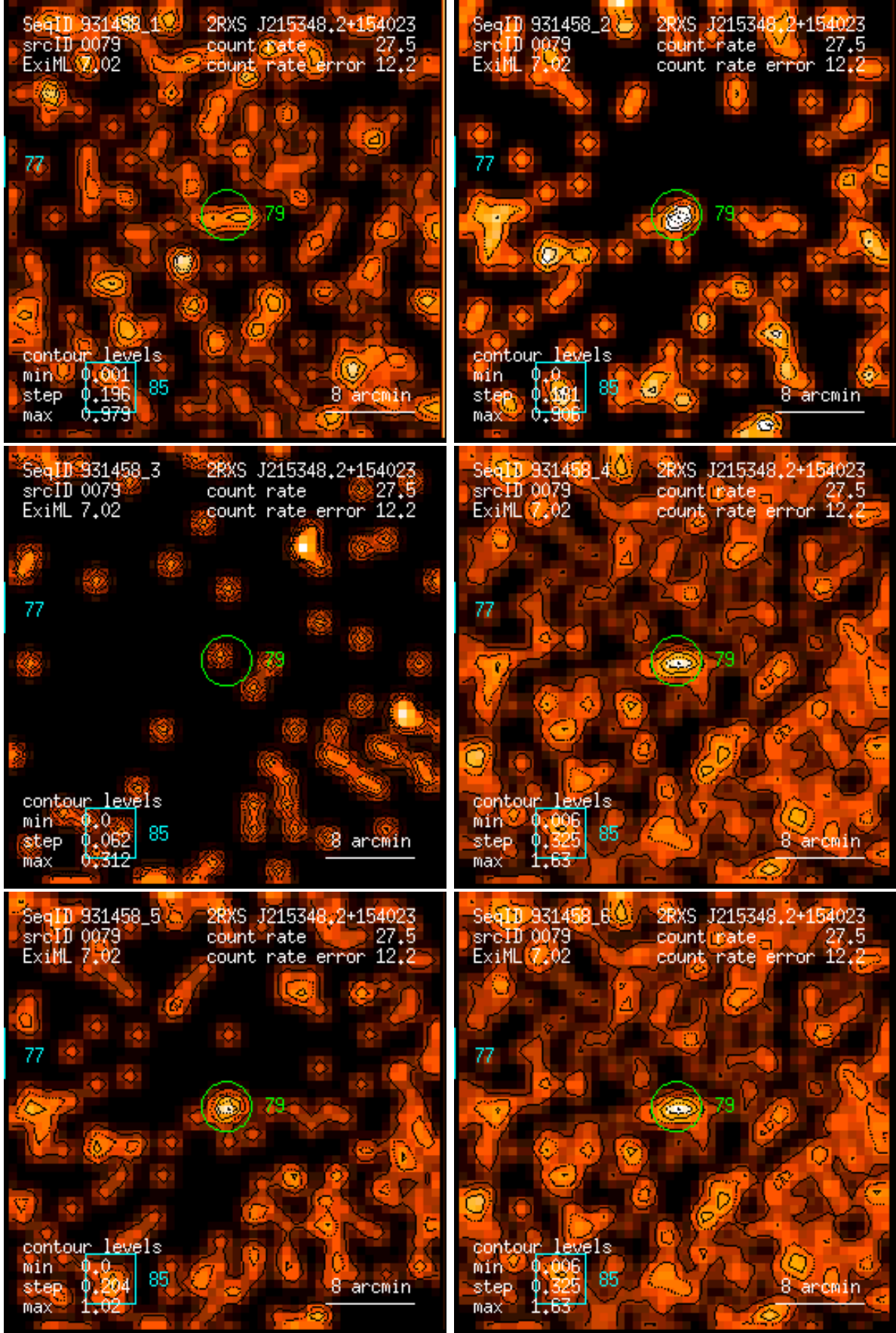
Figure 79: RASS 931458: detection 0079: band rate images, Gaussian filter: (1) PSPC channels 11 – 41, (2) 52 – 90, (3) 91 – 201, (4) 11 – 235, (5) 52 – 201, (6) 11 – 201. Broad band rates in counts/ks. Band rate contour levels in counts/ks/arcmin 2 .
