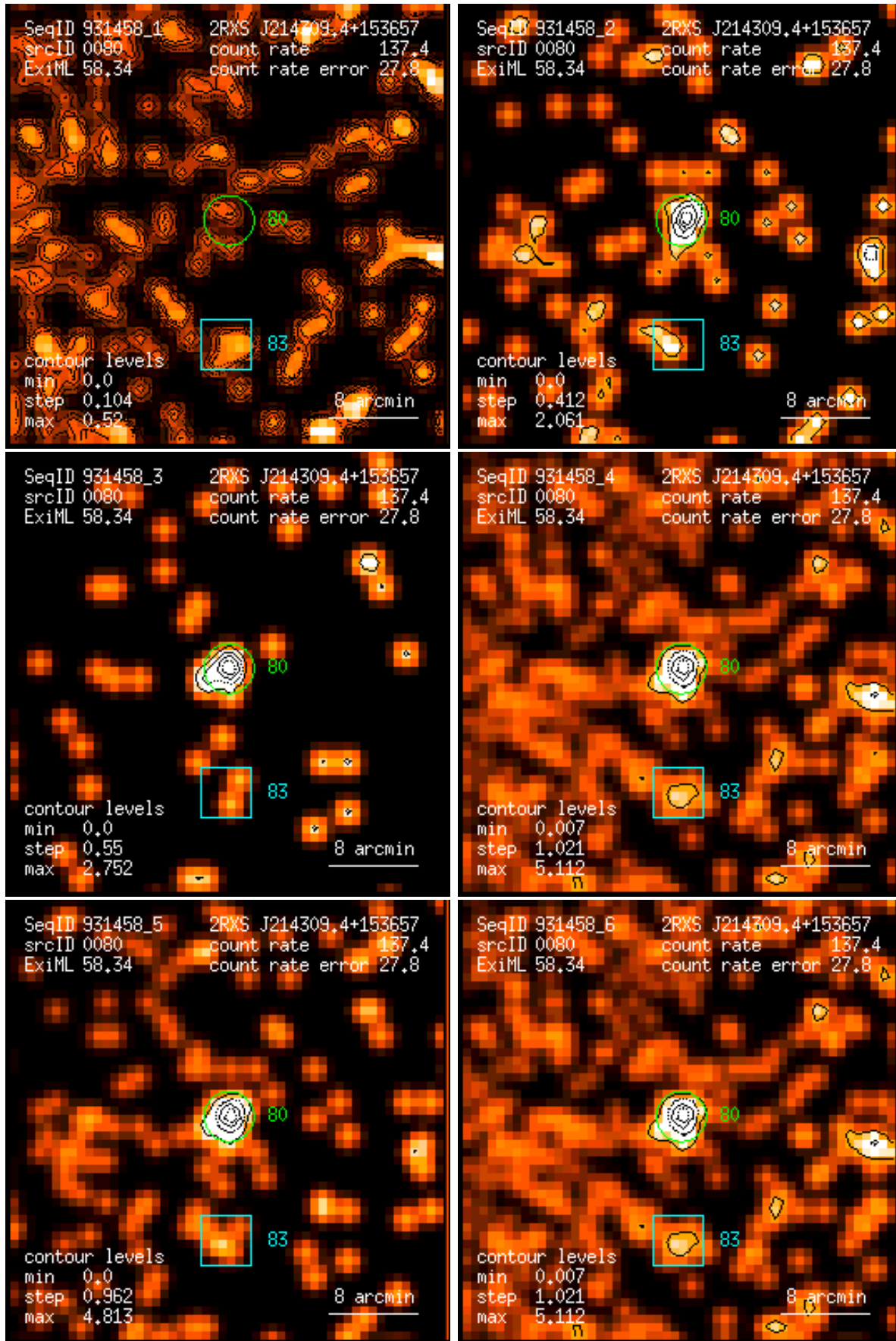
Figure 80: RASS 931458: detection 0080: band rate images, Gaussian filter: (1) PSPC channels 11 – 41, (2) 52 – 90, (3) 91 – 201, (4) 11 – 235, (5) 52 – 201, (6) 11 – 201. Broad band rates in counts/ks. Band rate contour levels in counts/ks/arcmin 2 .
