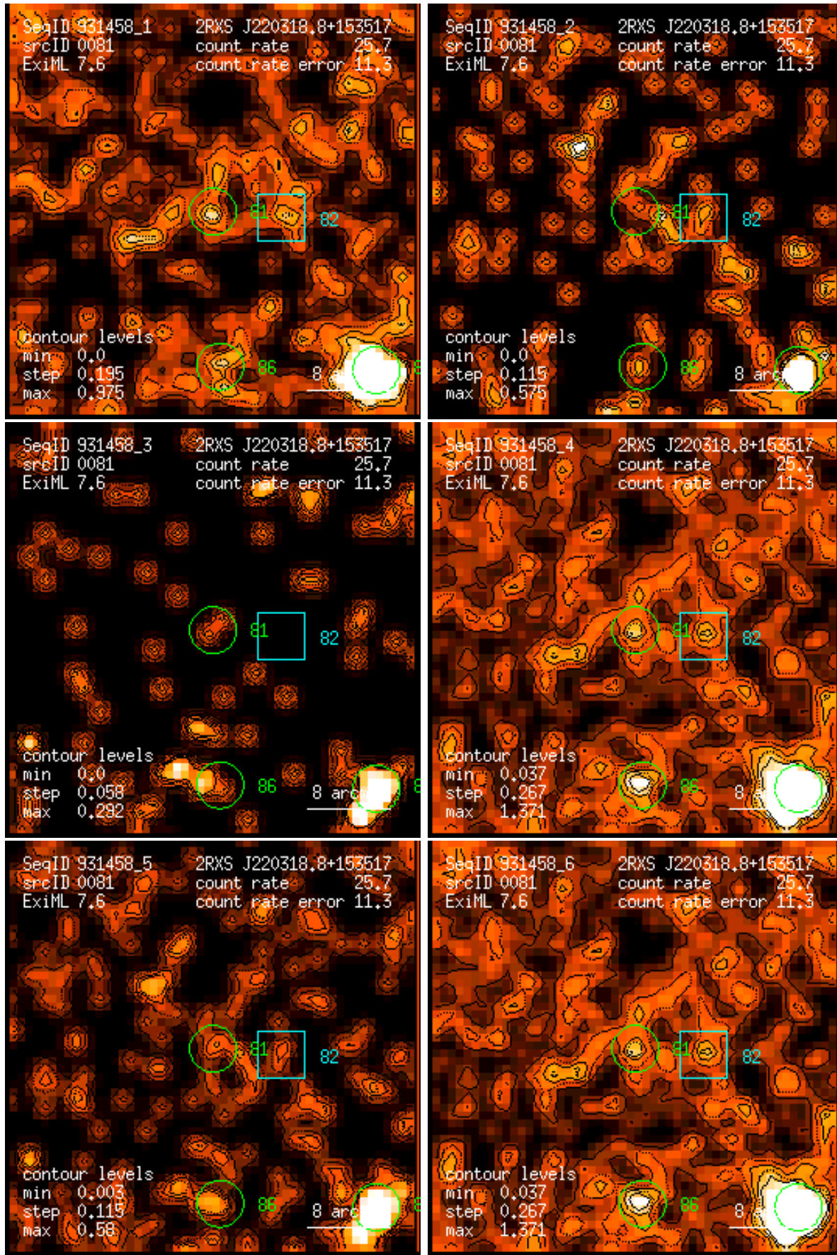
Figure 81: RASS 931458: detection 0081: band rate images, Gaussian filter: (1) PSPC channels 11 – 41, (2) 52 – 90, (3) 91 – 201, (4) 11 – 235, (5) 52 – 201, (6) 11 – 201. Broad band rates in counts/ks. Band rate contour levels in counts/ks/arcmin 2 .
