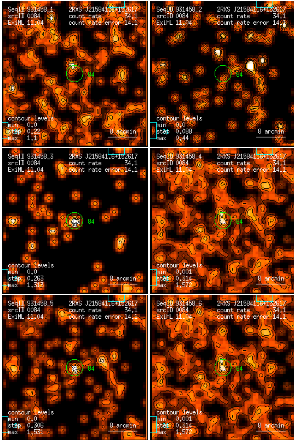
Figure 84: RASS 931458: detection 0084: band rate images, Gaussian filter: (1) PSPC channels 11 – 41, (2) 52 – 90, (3) 91 – 201, (4) 11 – 235, (5) 52 – 201, (6) 11 – 201. Broad band rates in counts/ks. Band rate contour levels in counts/ks/arcmin 2 .
