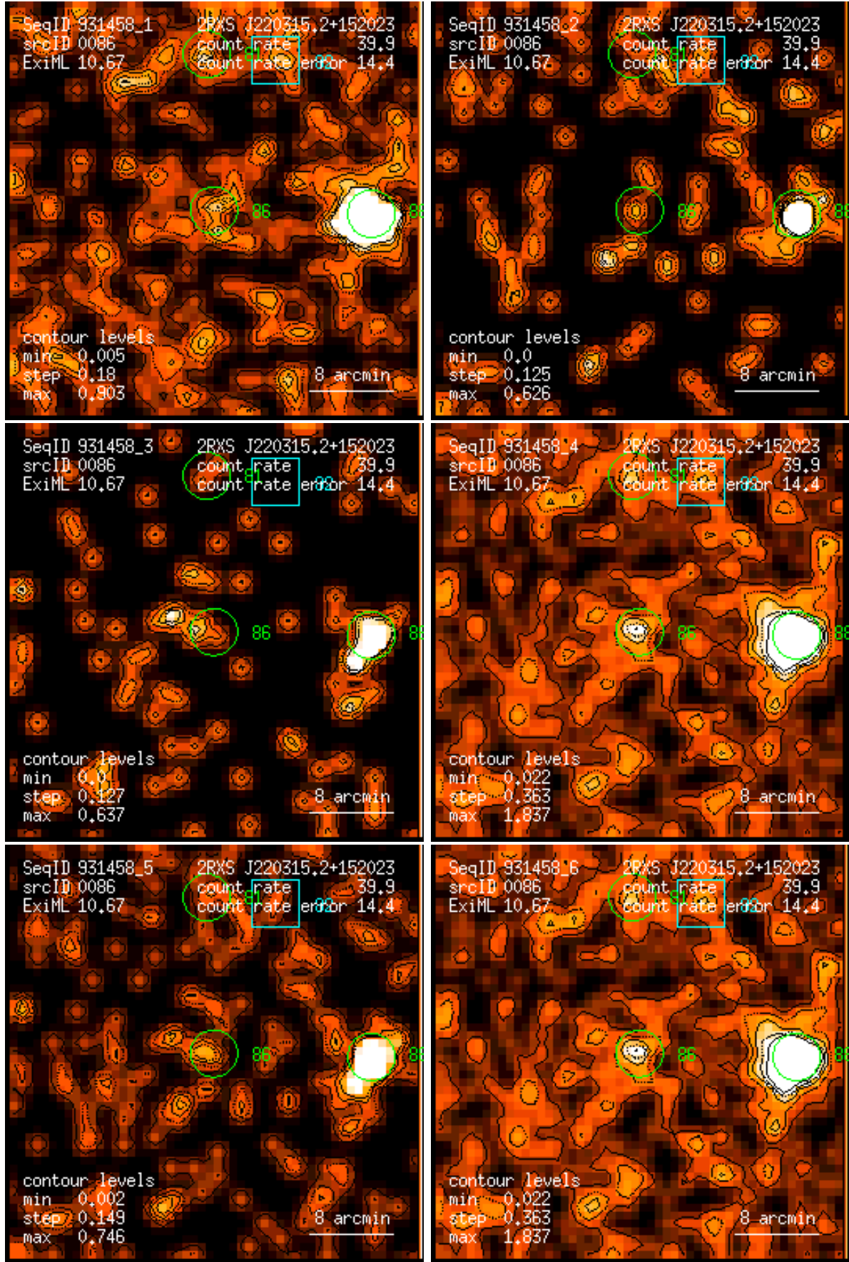
Figure 86: RASS 931458: detection 0086: band rate images, Gaussian filter: (1) PSPC channels 11 – 41, (2) 52 – 90, (3) 91 – 201, (4) 11 – 235, (5) 52 – 201, (6) 11 – 201. Broad band rates in counts/ks. Band rate contour levels in counts/ks/arcmin 2 .
