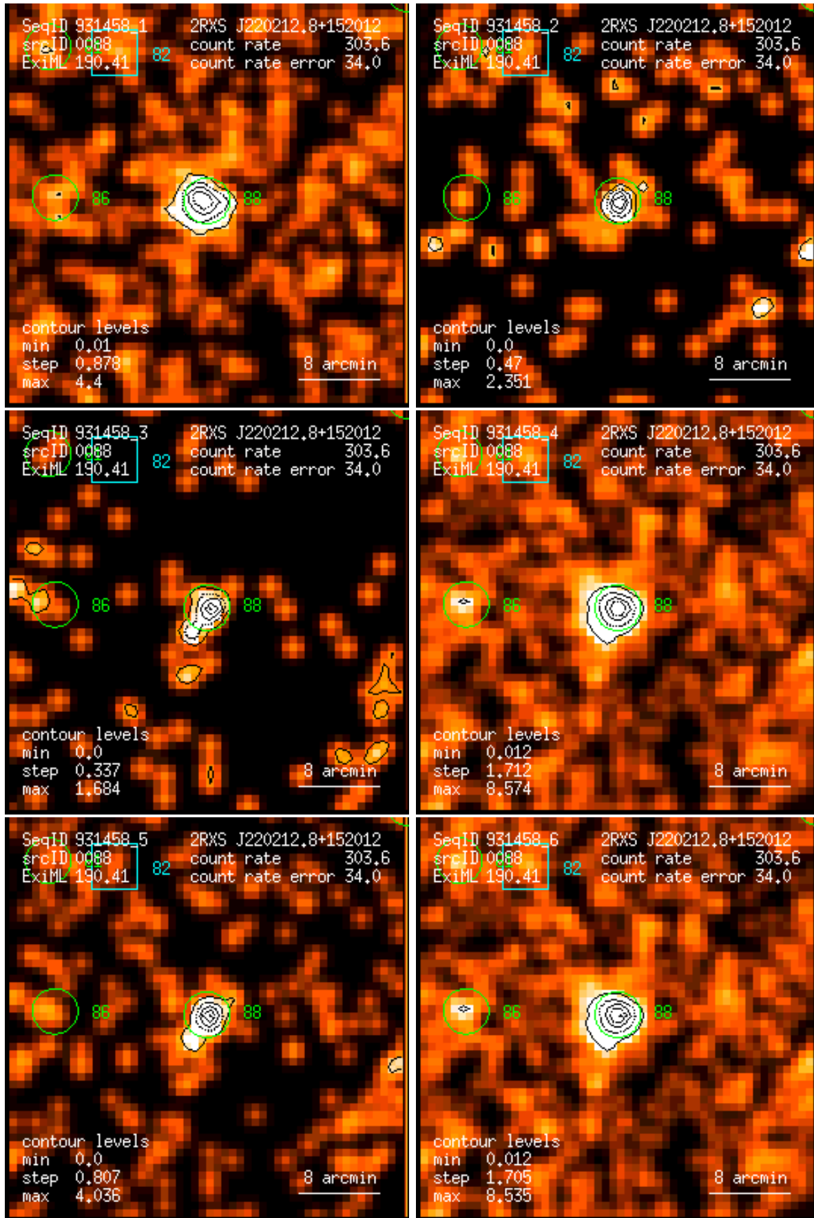
Figure 88: RASS 931458: detection 0088: band rate images, Gaussian filter: (1) PSPC channels 11 – 41, (2) 52 – 90, (3) 91 – 201, (4) 11 – 235, (5) 52 – 201, (6) 11 – 201. Broad band rates in counts/ks. Band rate contour levels in counts/ks/arcmin 2 .
