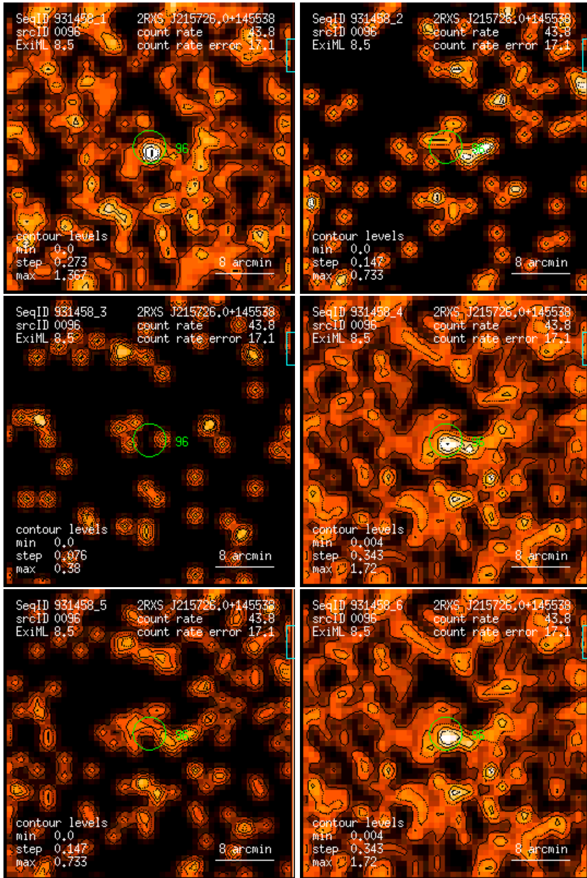
Figure 96: RASS 931458: detection 0096: band rate images, Gaussian filter: (1) PSPC channels 11 – 41, (2) 52 – 90, (3) 91 – 201, (4) 11 – 235, (5) 52 – 201, (6) 11 – 201. Broad band rates in counts/ks. Band rate contour levels in counts/ks/arcmin 2 .
