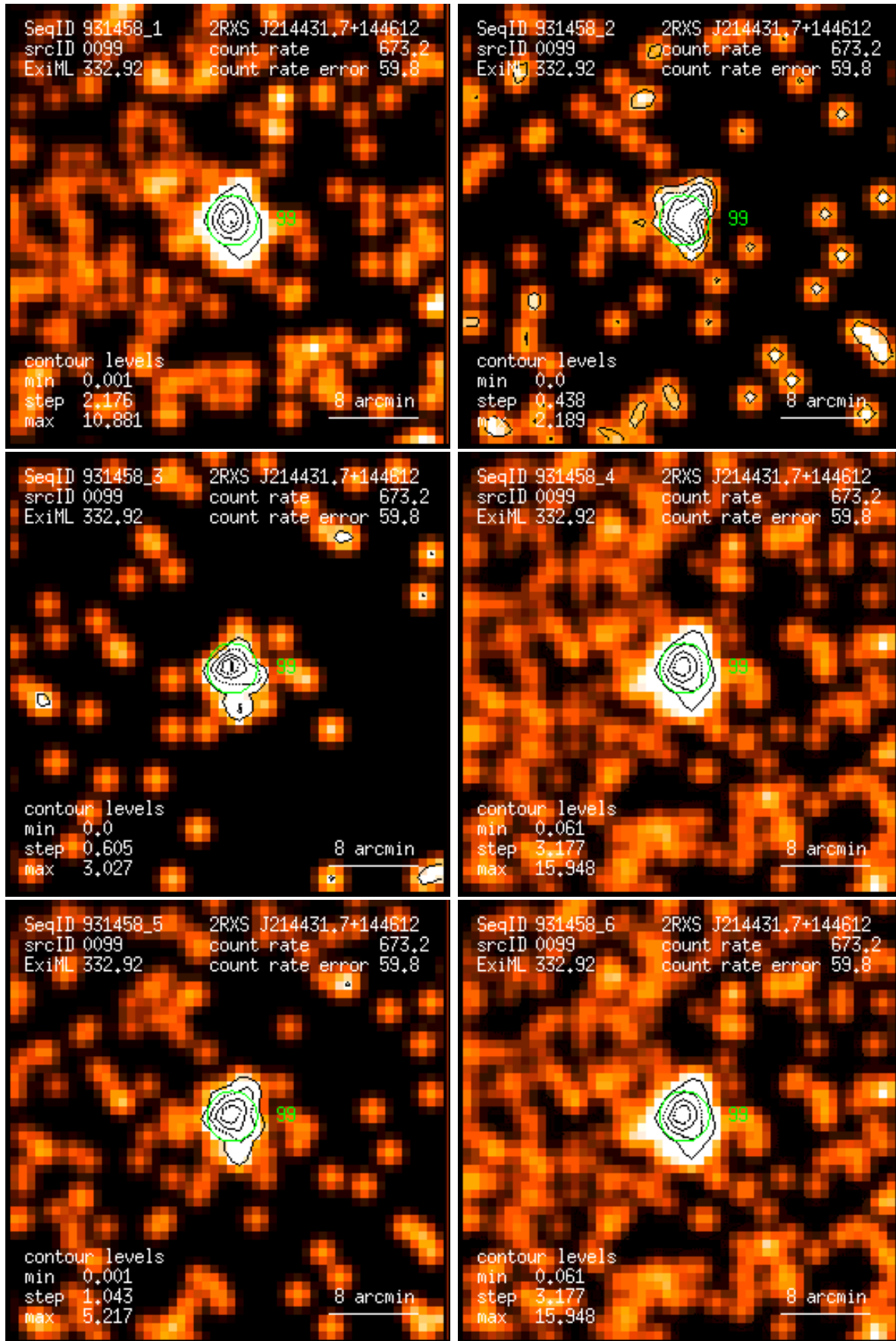
Figure 99: RASS 931458: detection 0099: band rate images, Gaussian filter: (1) PSPC channels 11 – 41, (2) 52 – 90, (3) 91 – 201, (4) 11 – 235, (5) 52 – 201, (6) 11 – 201. Broad band rates in counts/ks. Band rate contour levels in counts/ks/arcmin 2 .
